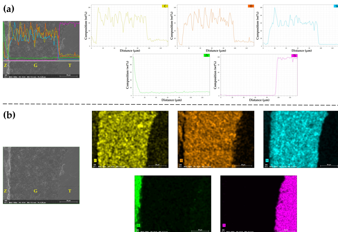
Figure 12. Line scan analysis and elemental mapping analysis at the same cross-sectional bonding interface for the NTP group in thermocycling. (a) Line scan analysis shows the distribution of each element along the white straight line marked in the FE-SEM image. (b) Elemental mapping analysis shows the presence of each element through color differences. Z, Zirconia surface. G, G-CEM LinkAce. T, Titanium abutment. C, Carbon. O, Oxygen. Si, Silicon. Zr, Zirconium. Ti, Titanium.
