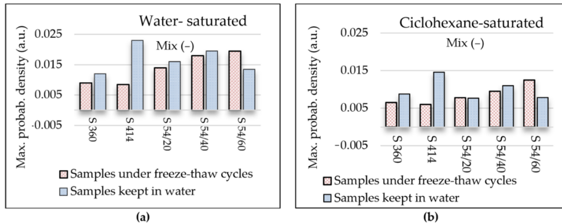
Figure 7. Maximum value of the probability density corresponding to the gel pores in the case of water saturated (a) and cyclohexane saturated (b) samples.
