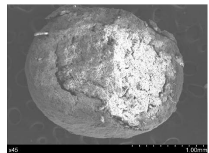
(b) Microcapsules after rupture
