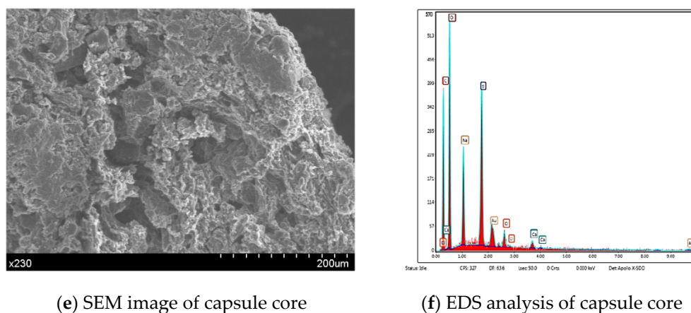
Figure 3. (a–f) SEM and EDS analysis of microcapsules.
