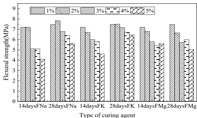
(a) Flexural strength
