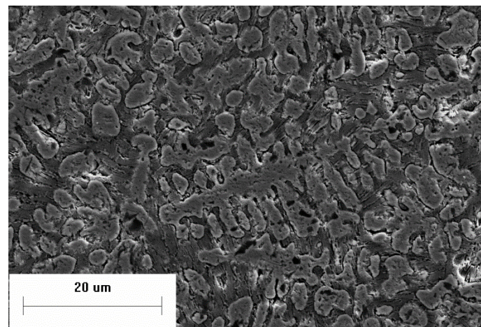
Figure 6. Powder microstructure ( d = 280\text{ }\mu\text{m} ).
