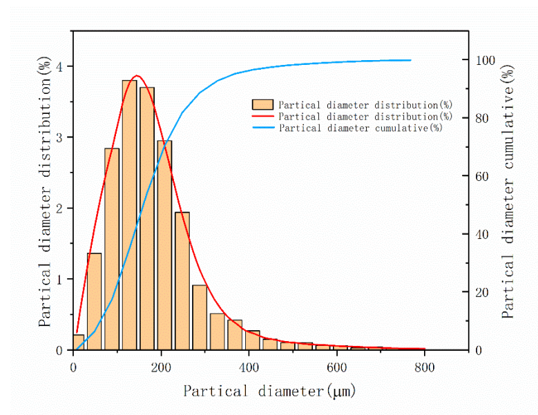
Figure 2. Particle size distribution of original powder.
