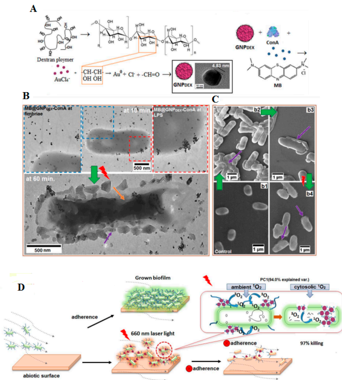
Figure 7. Schematic representation of the synthesis of dextran capped AuNPs (A). TEM image of localized MB@GNPDEX-ConA on K. Pneumoniae -12 bacterial surface and treatment. The schematic displays the cytological mass with accumulated conjugates (yellow arrow) and cell surface discomposure (B). The uniform morphology of bacterial aggregation and control cells according to concanavalin A (ConA)-mediated connection of conjugates (C). With light irradiation, the singlet oxygen produces ambient ^1\text{O}_2 and cyto \text{O}_2 , however, the cytosolic singlet oxygen influence the bactericidal effect and the absence of adherence through ambient oxygen. Singlet oxygen around the bacterial cells decreases the adherence ability (D) [158] Reprinted with permission from Elsevier. Table 2 displays other examples of the application of Au NPs in antimicrobial resistance activity (AMR).
