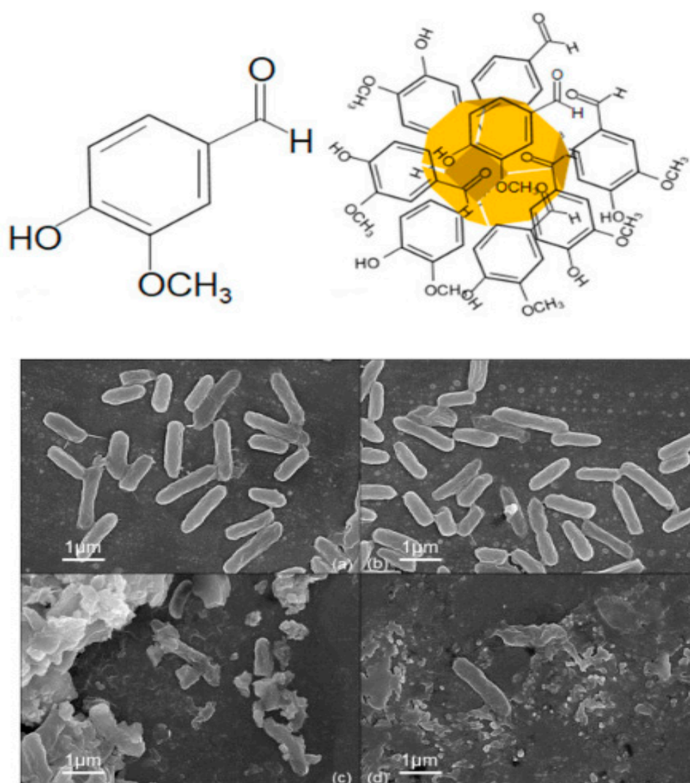
Figure 2. Schematic illustration of synthesized VAuNPs by vanillin (the above illustration); FESEM image of P. aeruginosa in untreated, in presence of the 50 µg/mL of VAuNPs, Meropenem-200 µg/mL (c), and (d) Meropenem (20 µg/mL) and VAuNPs (50 µg/mL) (the below images) [43]. Reprinted with permission from Elsevier.
