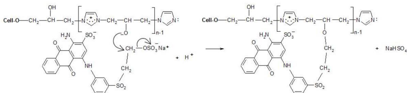
Figure 10. Proposed mechanism of dyeing [Cell-O-IME] + Cl - with RB 19 (mono-VS reactive dye).
