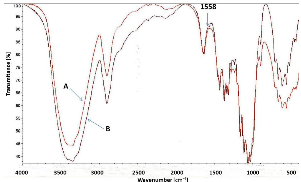
Figure 8. FT-IR spectrum of Cell-OH (A) and [Cell-O-IME] + Cl - (B)-(1558 cm -1 —specific wavenumber. for C = N bond in imidazole ring).
