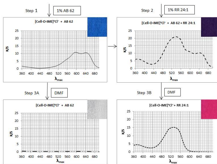
Figure 15. The diagrams presented the running process of mixed dyeing of [Cell-O-IME] + Cl - with RR 24:1 and AB 62 and the extraction results with DMF.
