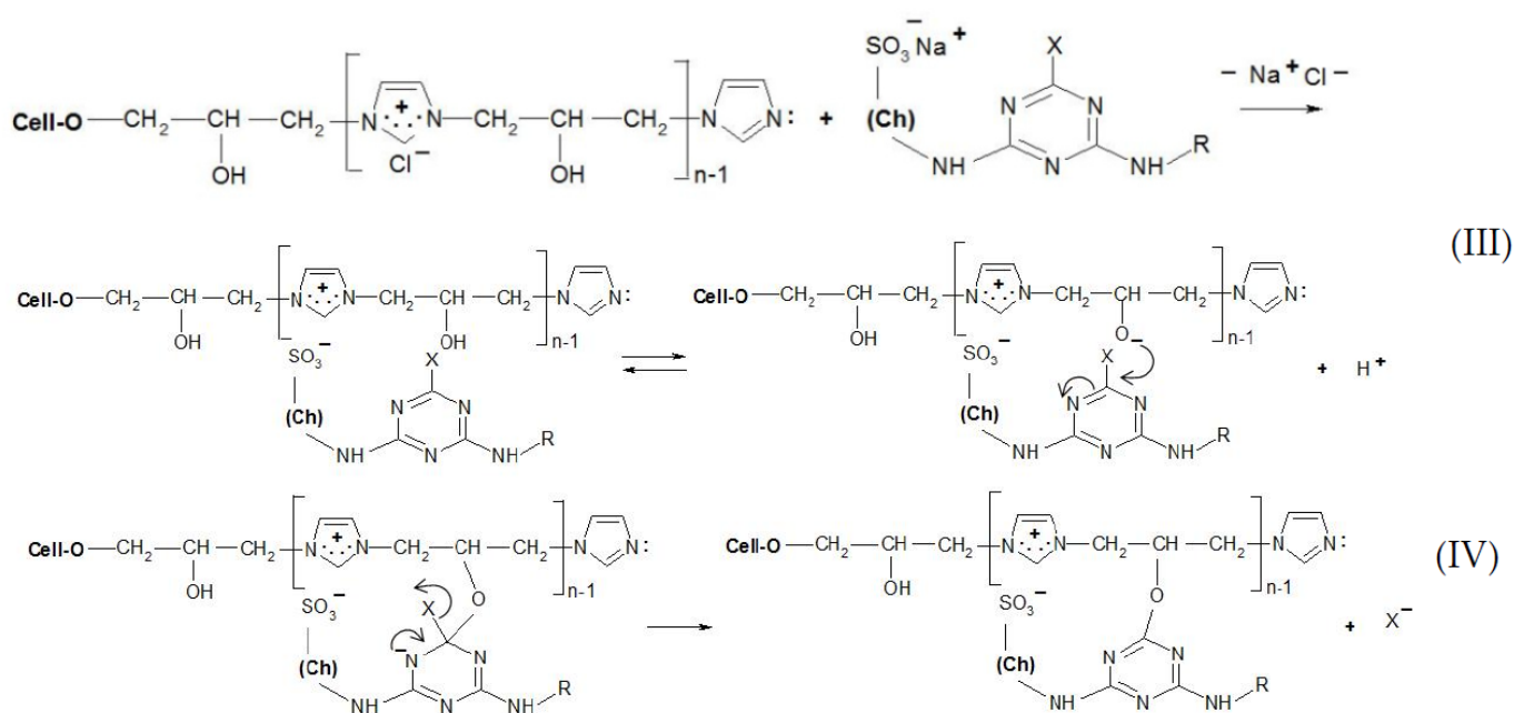
Figure 9. Proposed mechanism of the dyeing [Cell-O-IME] + Cl - with triazine dyes: (III) ionic formation bonds on the fibre and dissociation of a hydroxyl group in ionic pair: cationised cotton + reactive dye on the fibre, (IV) substitution reaction with formation of a covalent bond between reactive dye and nucleophile of the hydroxyl group where: Ch—chromophore of RR 24:1, RB 160, RR 221 and RR 274, R—different chemical substituents in the chemical structure above dyes X—nicotinic acid for RR 221, halogen for the other dyes.
