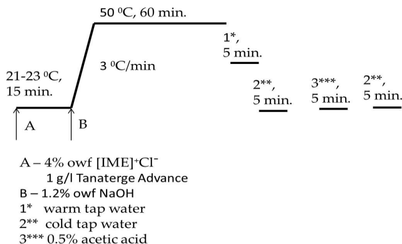
Figure 3. Diagram of cationisation process of cellulose with [IME] + Cl - .
