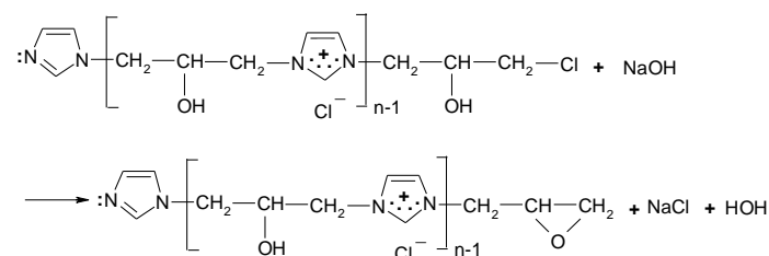
Figure 5. Scheme for creating a reactive form of [\text{IME}]^+\text{Cl}^- .
