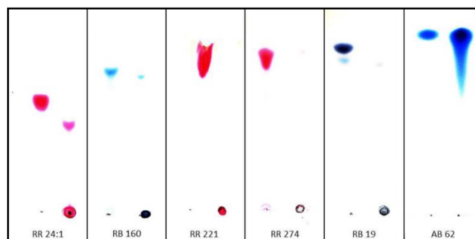
Figure 11. TLC chromatography coloured compounds obtained in reactions between reactive dyes and acid dye with [IME] + Cl - (left side—analysed dye, right side—the reaction product of dye with [IME] + Cl - ).
