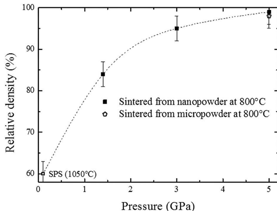
Figure 12. Density evolution with pressure in recovered \alpha - \text{Al}_2\text{O}_3 ceramics sintered at 800 °C from \gamma - \text{Al}_2\text{O}_3 with nano or micro-sized grains. The first symbol at lowest pressure corresponding to conventional SPS (100 MPa). (Figure adapted from [61]).
