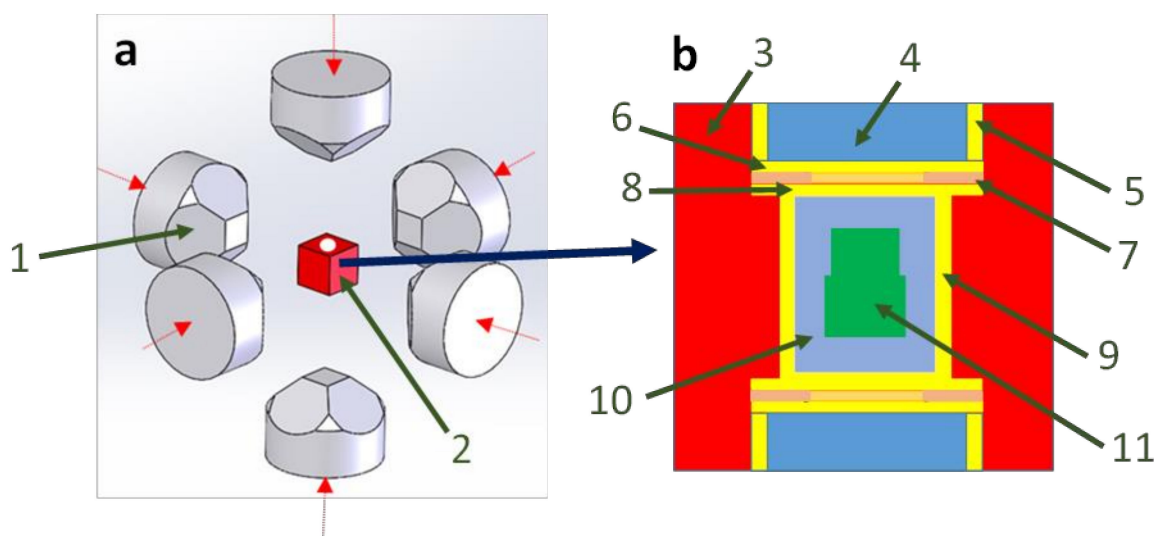
Figure 7. (a) Schematic of cubic press assembly showing the six opposite WC anvils and the cube assembly in the middle; (b) Enlargement of the associated cubic reaction chamber. (1) WC anvils. (2) Cubic reaction chamber. (3) Gasket material. (4) “Synthetic gasket material”. (5) Steel electrode. (6) First metallic disk. (7) Baffle. (8) Second metallic disk. (9) Graphite heater. (10) Salt capsule. (11) Metallic capsule where the sample is placed. The red arrows indicate compression axes. Adapted from [22,54].
