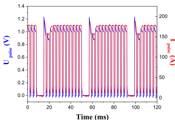
Figure 14. SPS pulse pattern, with an On:Off setting of 12:2, delivered using the homemade pulse generator to the tabletop HP-SPS.
