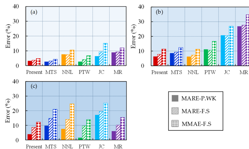
Figure 6. Three statistical average errors of model predictions within (a) \dot{\epsilon} \leq 10^3 \text{ s}^{-1} , (b) 10^3 \text{ s}^{-1} < \dot{\epsilon} \leq 10^4 \text{ s}^{-1} , and (c) \dot{\epsilon} > 10^4 \text{ s}^{-1} : MARE-P.WK, MARE-F.S, and MMAE-F.S.
