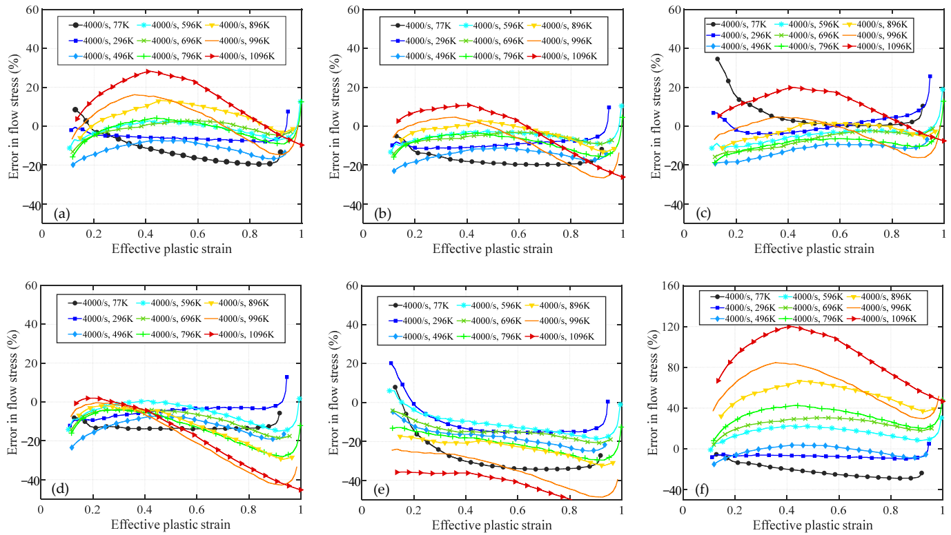
Figure 5. The relative error curve between the predicted values of models and the experimental results over a wide range of temperatures at a strain rate of 4000 \text{ s}^{-1} . The models are (a) Present, (b) MTS, (c) NNL, (d) PTW, (e) JC, and (f) MR.
