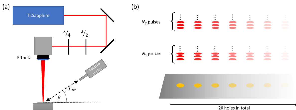
Figure 3. Experimental setup. (a) The beam of a Ti:Sapphire laser with a wavelength of 800 nm and a pulse repetition rate of 1 kHz was focused on a sample of stainless steel by means of an F-theta lens, leading to a peak irradiance of 1.1 \cdot 10^{14} \text{ W/cm}^2 on the initially plane surface. The spectrometer was placed at a distance of 35 cm from the processing region. (b) A total of 20 holes were processed for each measurement. All holes were repeatedly processed with the same number N_i of pulses, and the X-ray emission was measured separately for each processing step i . Hence, every measurement corresponds to the emission from a specific depth z_{hi} of the drilled holes.
