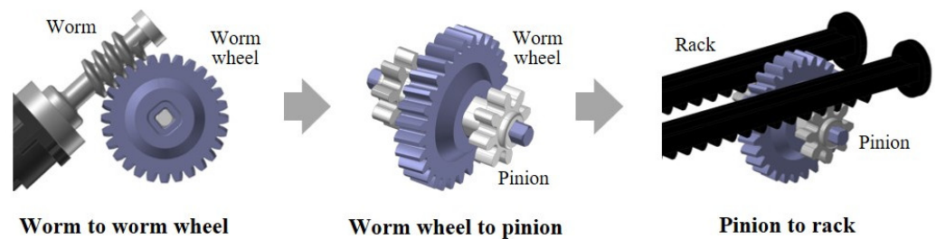
Figure 2. Power transmission mechanism.
