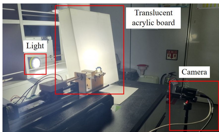
Figure 7. Video recording equipment.
