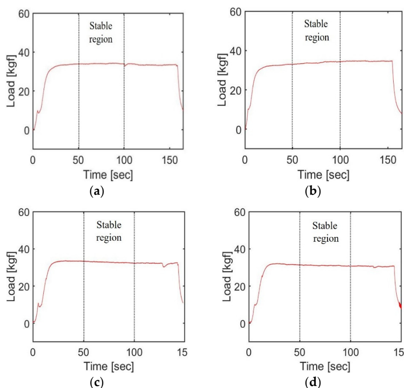
Figure 14. Results of total extrusion load of light type impression materials; (a) Mixing motor off, 1st test; (b) Mixing motor off, 2nd test; (c) Mixing motor on, 1st test; (d) Mixing motor on, 2nd test.
