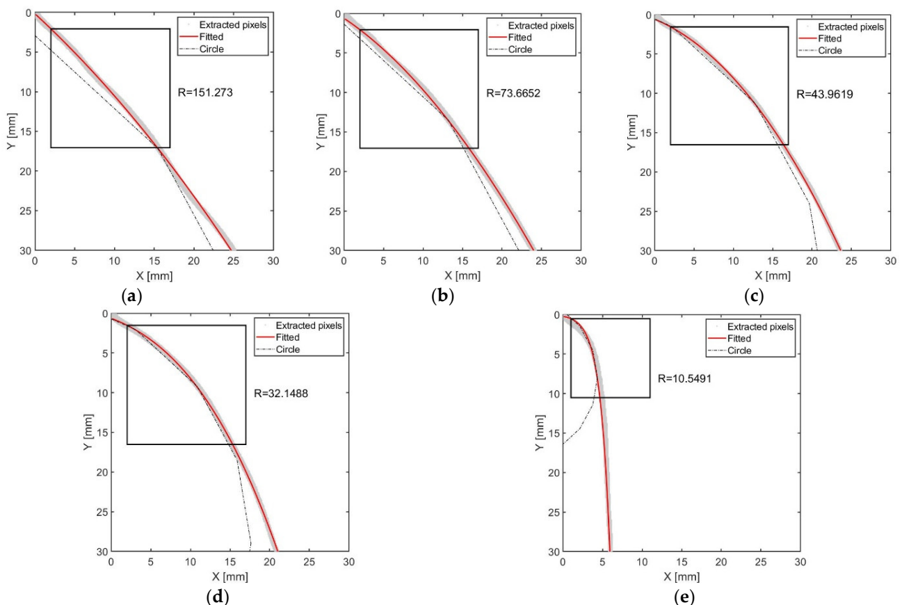
Figure 13. Graphs of extruded the impression material trajectory using image processing (2nd test): (a) 0.8 mm/s; (b) 0.7 mm/s; (c) 0.6 mm/s; (d) 0.5 mm/s; (e) 0.4 mm/s.
