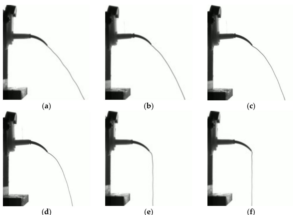
Figure 11. Impression material extrusion trajectory depending on pressurization speed: (a) 0.8 mm/s; (b) 0.7 mm/s; (c) 0.6 mm/s; (d) 0.5 mm/s; (e) 0.4 mm/s; (f) 0.3 mm/s.
