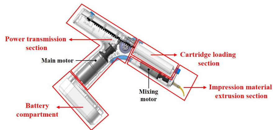
Figure 1. Structure of dental impression material electric dispenser.
