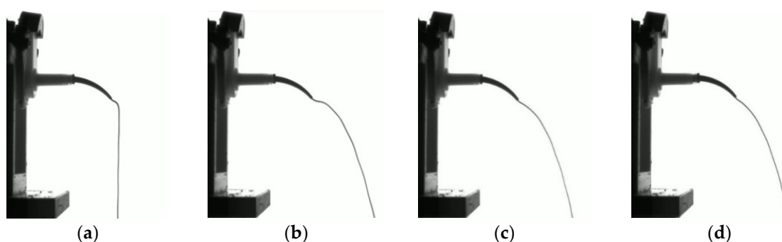
Figure 10. Impression material extrusion behavior over time (pressurization speed: 0.5 mm/s): (a) After 10 s; (b) After 30 s; (c) After 50 s; (d) After 70 s.
