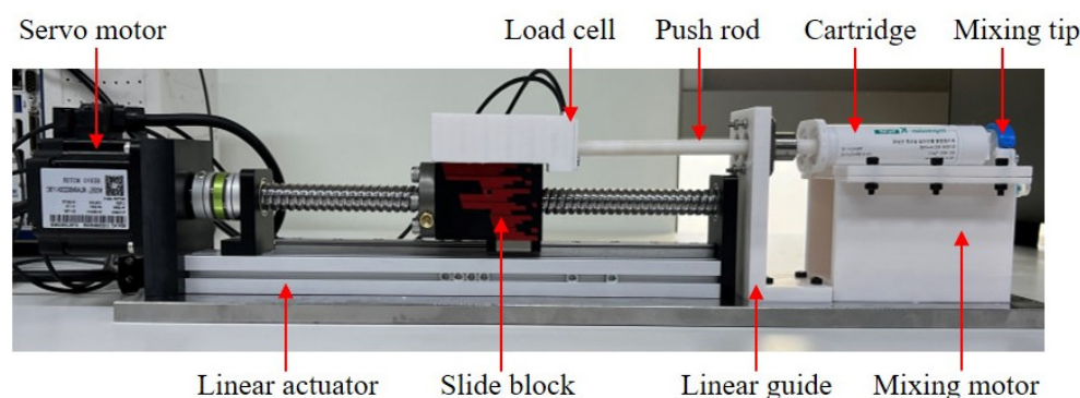
Figure 3. Structure of load measurement system testbed.
