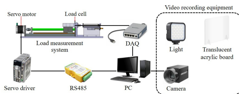
Figure 4. Schematic diagram of experimental setup.
