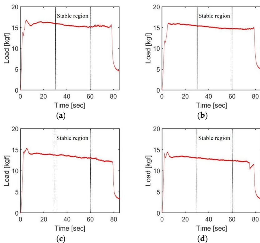
Figure 9. Results of extrusion load using medium body impression materials: (a) Mixing motor off, 1st test; (b) Mixing motor off, 2nd test; (c) Mixing motor on, 2nd test; (d) Mixing motor on, 2nd test.
