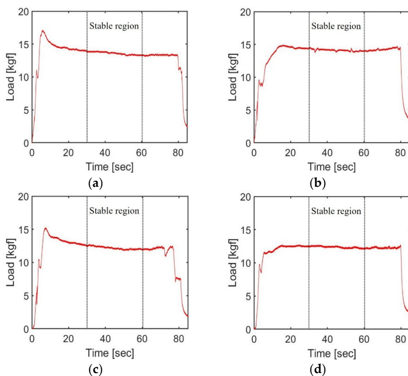
Figure 8. Results of extrusion load using light body impression materials: (a) Mixing motor off, 1st test; (b) Mixing motor off, 2nd test; (c) Mixing motor on, 2nd test; (d) Mixing motor on, 2nd test.
