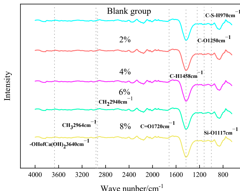
Figure 12. FTIR spectra of cement mortar with different emulsion dosages.
