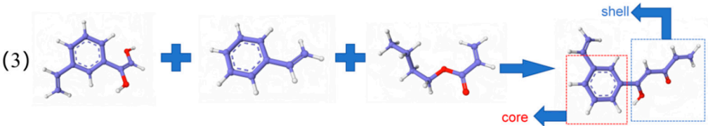
Figure 3. Schematic diagram of reaction and molecular structure of core-shell structure emulsion admixture.
