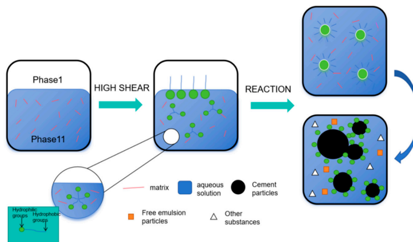
Figure 14. Schematic diagram of the microscopic action mechanism of core-shell emulsion in cement-based materials.
