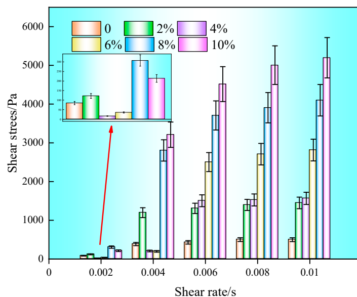
Figure 5. Shear rate vs. shear stress of cement mortar with different emulsion dosages.
