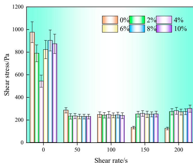
Figure 9. Shear stress vs. shear rate of cement mortar with different emulsion dosages.
