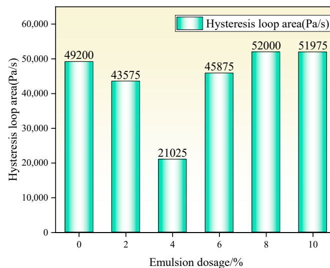
Figure 10. Hysteresis loop area vs. emulsion dosage.
