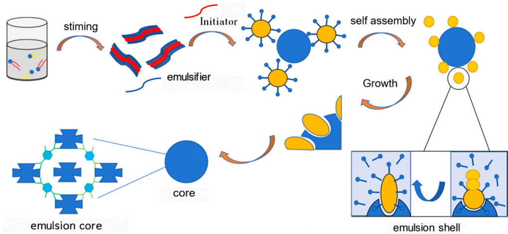
Figure 4. Schematic diagram of free radical polymerization mechanism of core-shell emulsion admixture.
