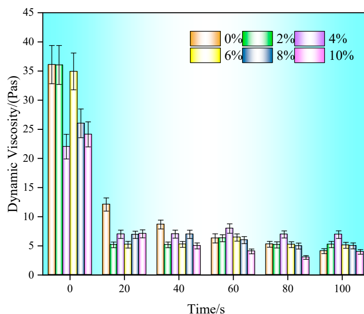
Figure 8. Dynamic viscosity vs. shearing time of cement mortar with different emulsion dosages.
