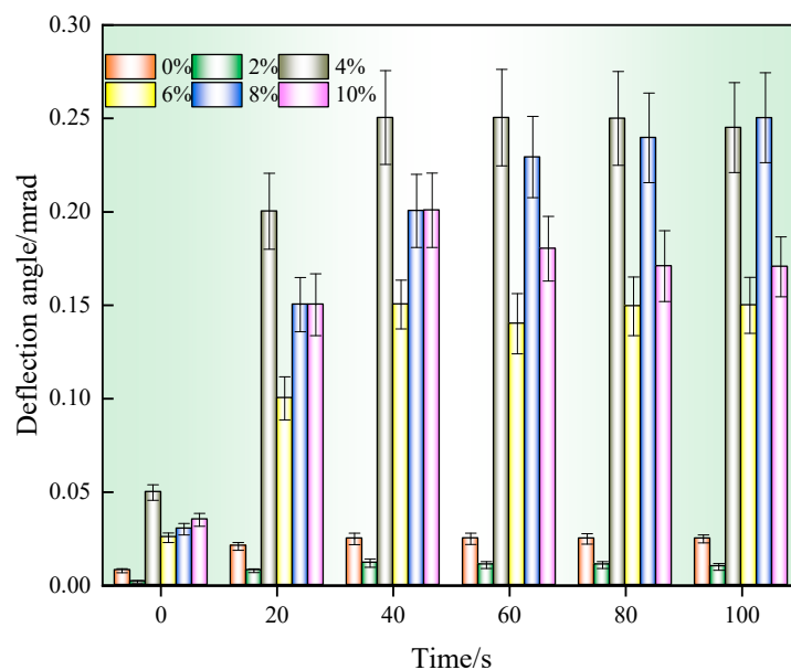
Figure 6. Deflection angle vs. time of cement mortar under different emulsion dosages.
