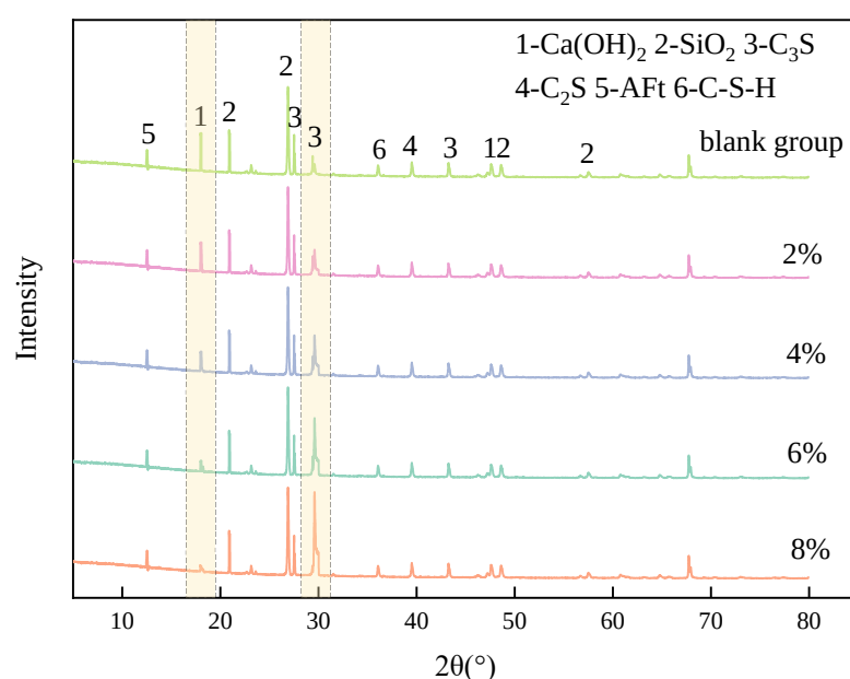
Figure 11. XRD patterns of cement mortar at different emulsion dosages.
