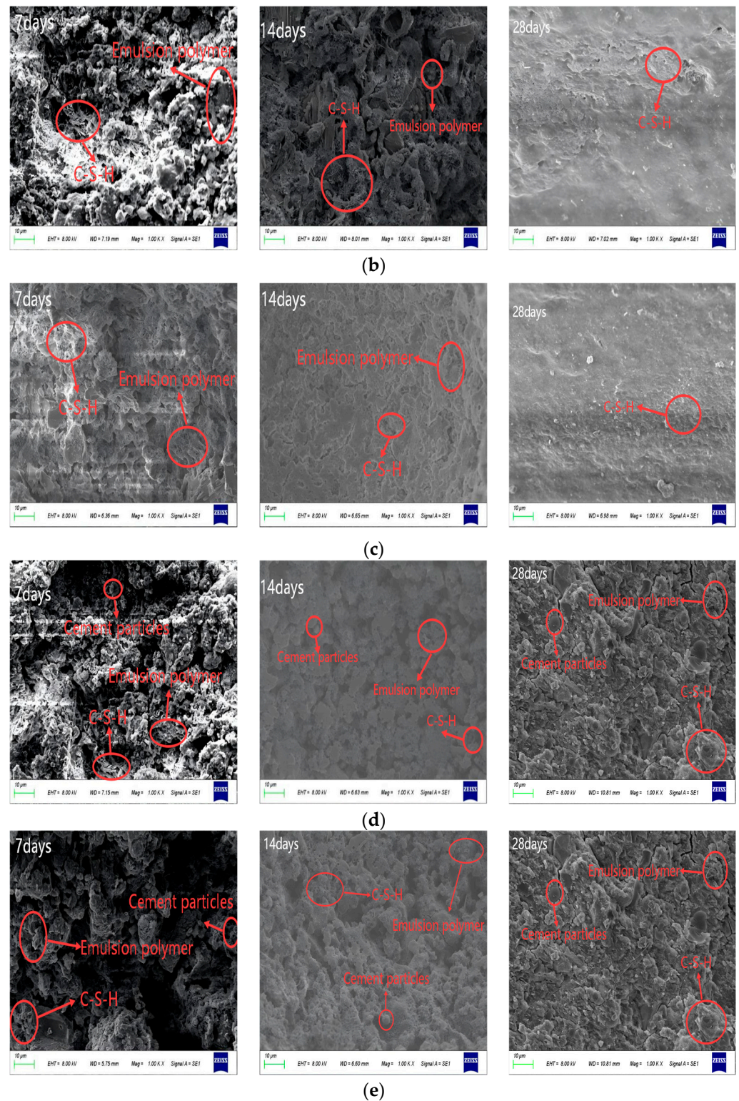
Figure 13. Microscopic morphology of cement mortar at different curing ages with different dosages of core-shell structured emulsion. (a) Microscopic morphology of ordinary cement mortar at different curing ages. (b) Microscopic morphology of cement mortar with 2% core-shell emulsion dosage at different curing ages. (c) Microscopic morphology of cement mortar with 4% core-shell structured emulsion at different curing ages. (d) Microscopic morphology of cement mortar with 6% core-shell structured emulsion at different curing ages. (e) Microscopic morphology of cement mortar with 8% core-shell structured emulsion at different curing ages.
