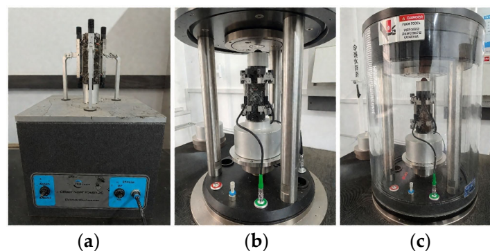
Figure 8. AMPT Testing Procedure: (a) Specimen Mounted with Positioning Pins. (b) Specimen Connected to Sensors. (c) Dynamic Modulus Test.
