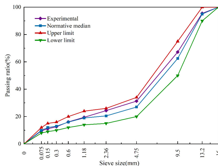
Figure 2. Gradation Curve of SMA-13.
