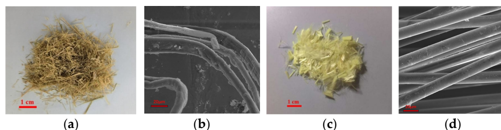
Figure 1. Appearance and Microscopic Morphology of Bamboo and Aramid Fibers: (a) appearance of bamboo fiber; (b) microscopic morphology of bamboo fiber; (c) appearance of aramid fiber; (d) microscopic morphology of aramid fiber.
