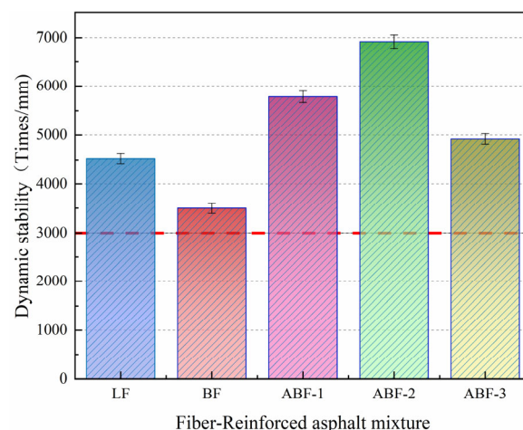
Figure 9. Dynamic Stability of Fiber-Reinforced SMA Mixtures.
