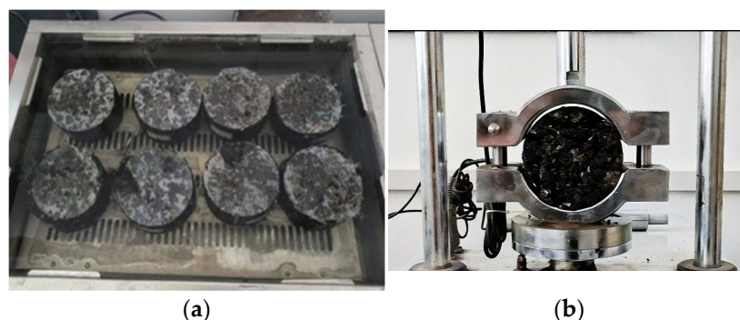
Figure 6. Water Bath Conditioning of Fiber-Reinforced Asphalt Mixtures and Marshall Stability Test: (a) Water Bath Conditioning of Asphalt Mixtures. (b) Marshall Stability Test.
