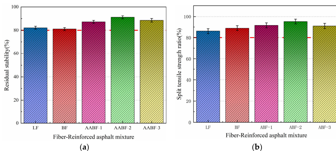
Figure 11. (a) Residual stability of asphalt mixtures. (b) Asphalt mixture split tensile strength ratio.
