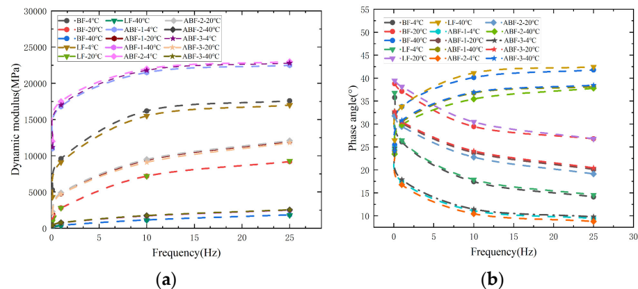
Figure 12. Dynamic Modulus and Phase Angle of Fiber-Reinforced Asphalt Mixtures: (a) dynamic modulus; (b) phase angle.
