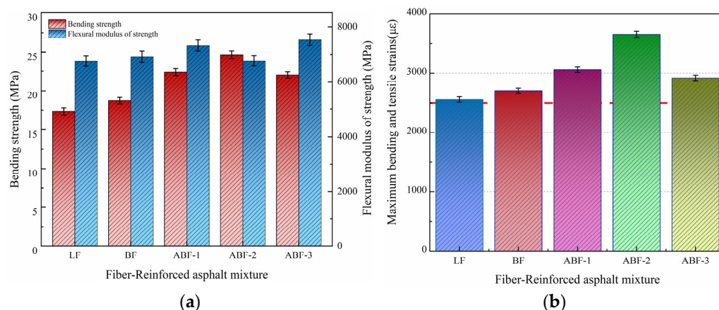
Figure 10. Results of low-temperature trabecular bending tests of asphalt mixtures: (a) asphalt mixture flexural strength and asphalt mixture flexural modulus results; (b) maximum bending tensile strain of the asphalt mixture.
