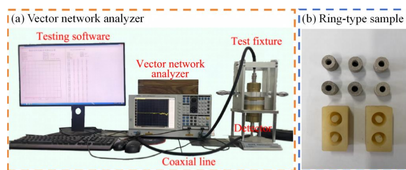
Figure 3. Experimental setup of microwave-absorbing properties.
