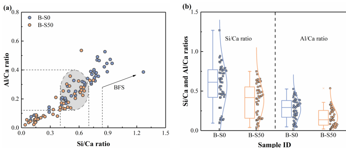
Figure 17. EDS point analysis: (a) Si/Ca vs. Al/Ca ratios; and (b) chemical compositions of gel hydrates.
