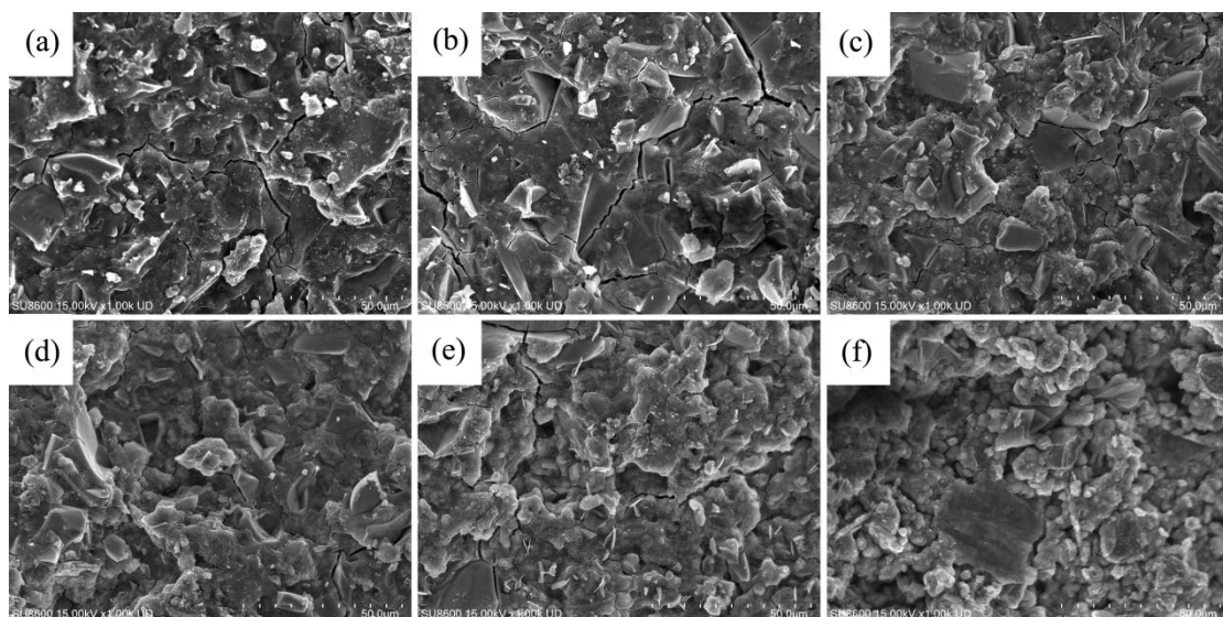
Figure 9. Microstructure of AAS with different SS dosages at 3 d: (a) 0%; (b) 10%; (c) 30%; (d) 50%; (e) 70%; and (f) 90%.
