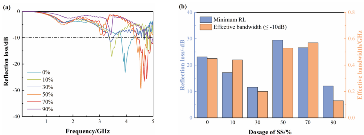
Figure 13. Microwave-absorbing properties of AAS with different SS dosages: (a) RL value; and (b) minimum RL and effective bandwidth.
