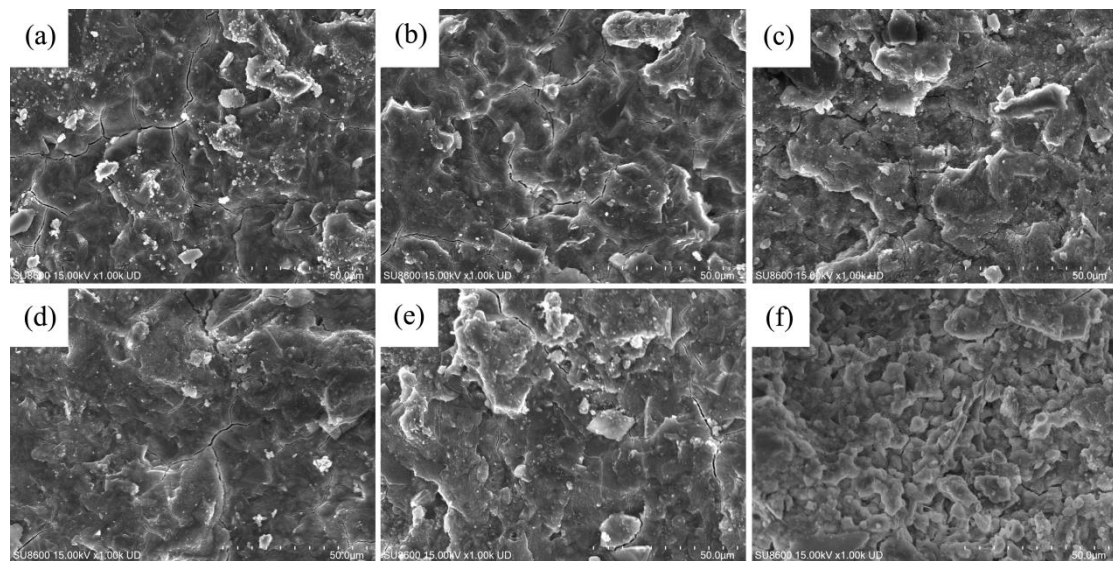
Figure 10. Microstructure of AAS with different SS dosages at 28 d: (a) 0%; (b) 10%; (c) 30%; (d) 50%; (e) 70%; and (f) 90%.
