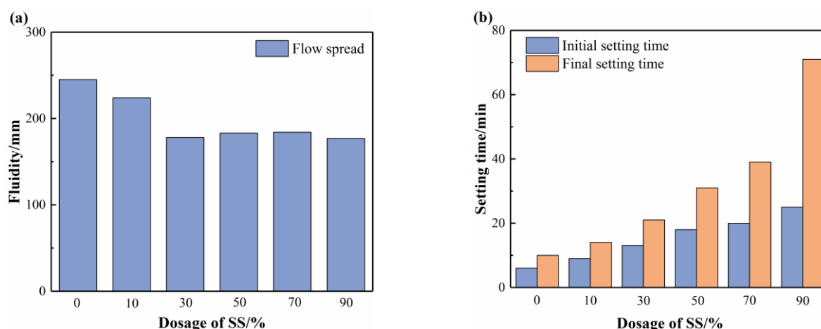
Figure 5. Workability of AAS with different SS dosages: (a) fluidity; and (b) initial and final setting times.
