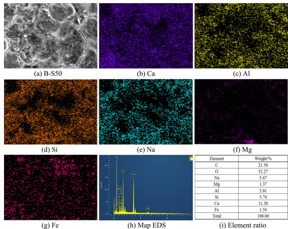
Figure 11. EDS analysis of B-S50.
