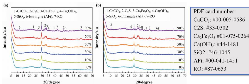
Figure 7. XRD pattern of AAS with different SS dosages: (a) 3 d; and (b) 28 d.
