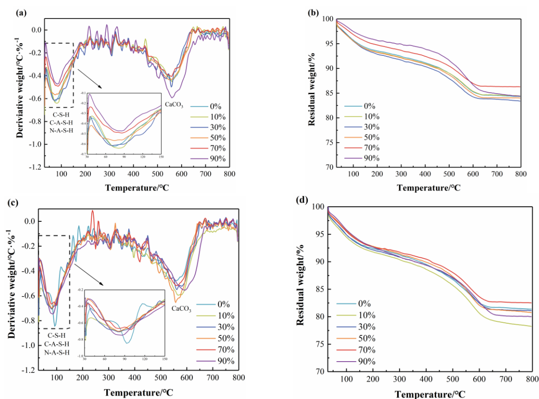
Figure 8. TG/DTG curve of AAS with different SS dosages: (a) and (b) for 3 d; and (c) and (d) for 28 d.
