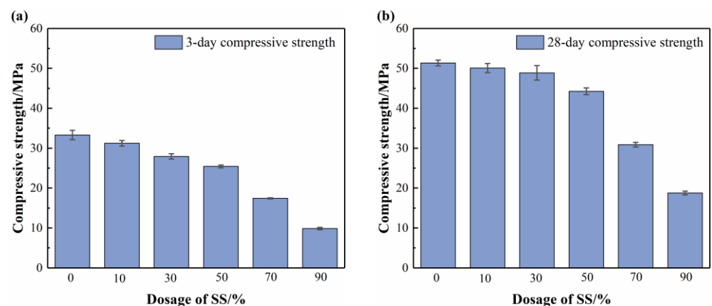
Figure 4. Compressive strength of AAS with different SS dosages: (a) 3 d; and (b) 28 d.
