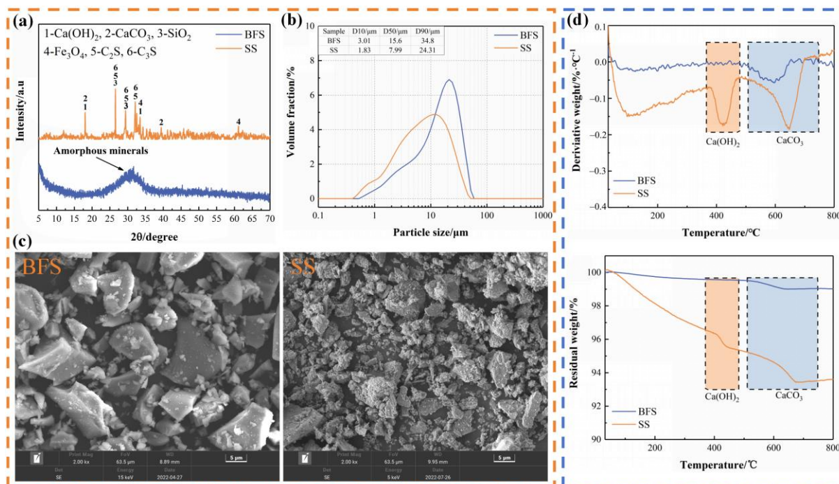
Figure 1. Basic performance of BFS and SS: (a) mineral compositions; (b) particle-size distributions; (c) microstructure; and (d) TG/DTG curves.
