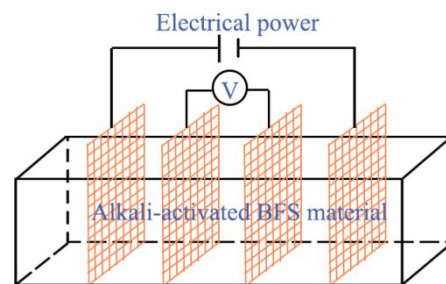
Figure 2. Schematic diagram of electrical resistivity test.
