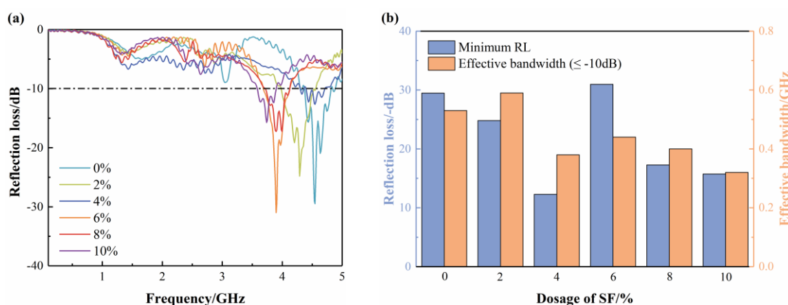
Figure 14. Microwave-absorbing properties of B-S50 with various SF dosages: (a) RL value; and (b) minimum RL and effective bandwidth.
