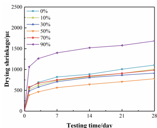
Figure 6. Drying shrinkage of AAS with different SS dosages.
