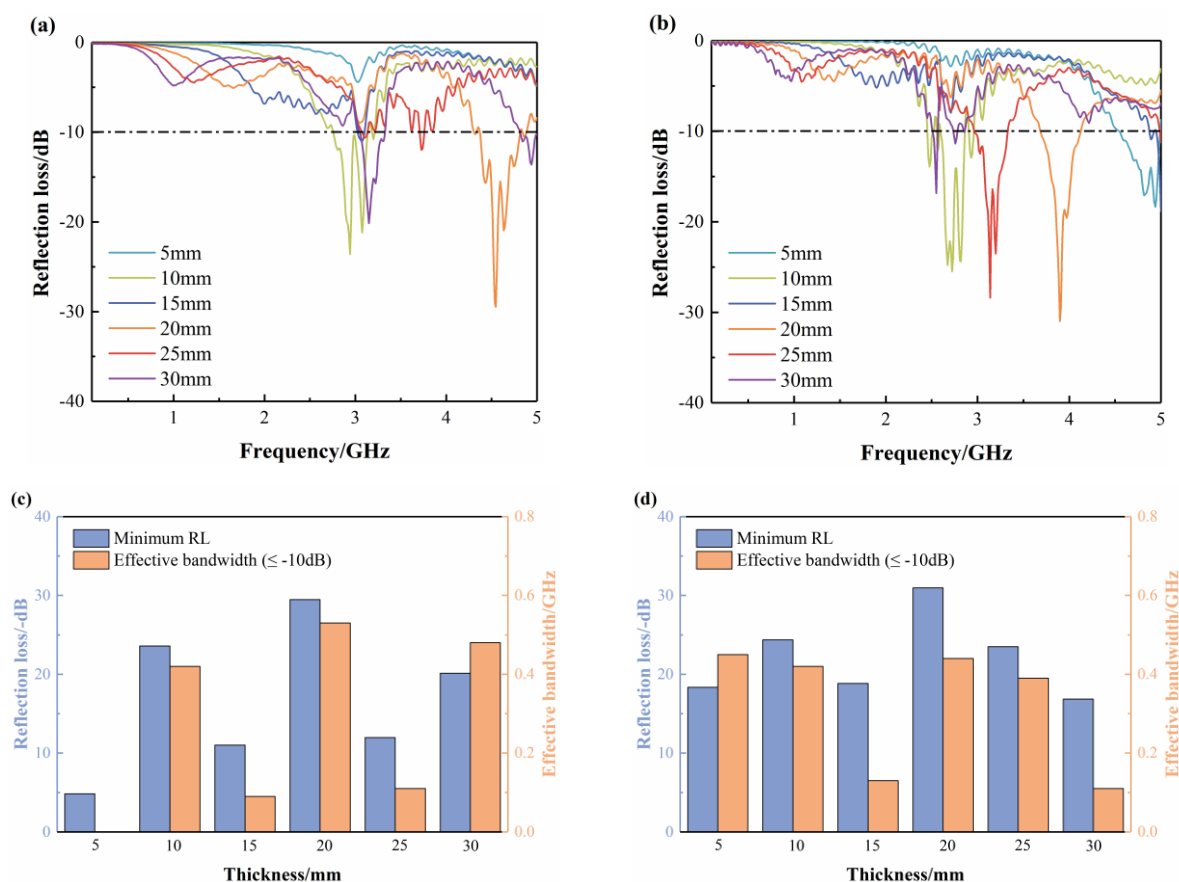
Figure 15. Microwave-absorbing properties of optimal sample with different thicknesses: (a) B-S50; (b) B-S50-6; and (c,d) minimum RL and effective bandwidth of B-S50 and B-S50-6.
