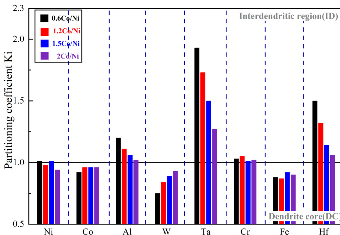
Figure 5. Dendritic Segregation Coefficient for Alloys with Different Co/Ni Ratios.
