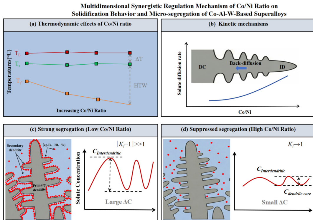
Figure 6. Schematic diagram illustrating the multidimensional synergistic evolution mechanism of solidification characteristics and microstructural segregation in alloys with different Co/Ni ratios.
