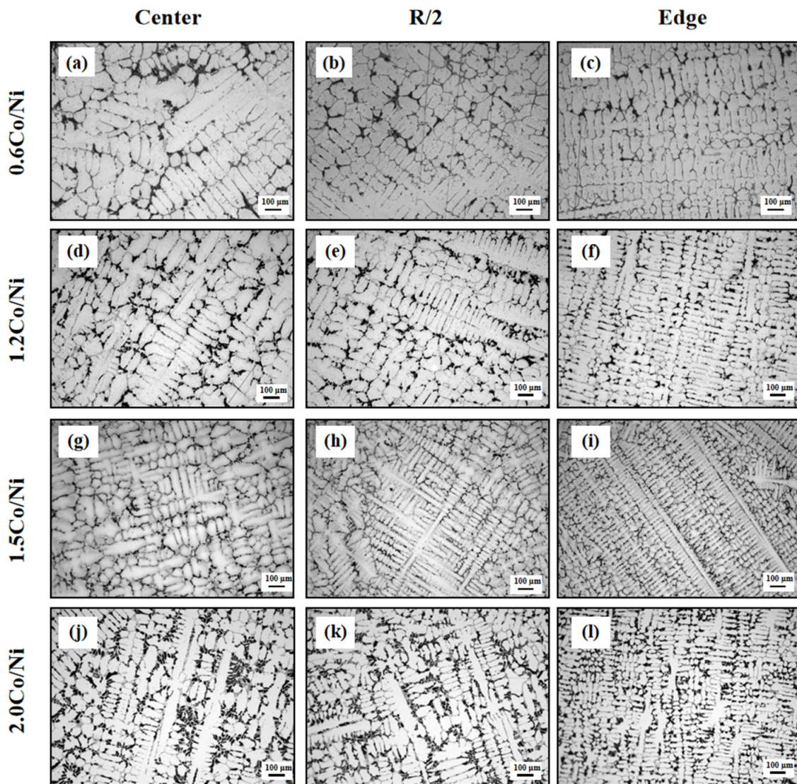
Figure 2. OM image showing the radial gradient of dendritic morphology (Center, R/2 position, and Edge) across ingots with varying Co/Ni ratios: (a–c) 0.6Co/Ni; (d–f) 1.2Co/Ni; (g–i) 1.5Co/Ni; (j–l) 2.0Co/Ni.
