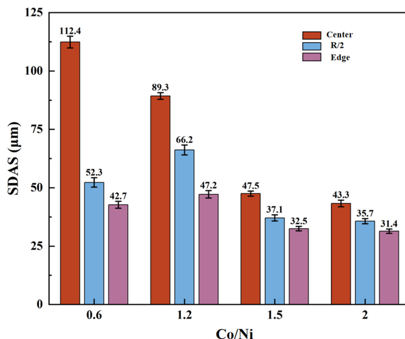
Figure 3. Variation Trends of SDAS (μm) in Different Regions of Alloys with Different Co/Ni Ratios.
