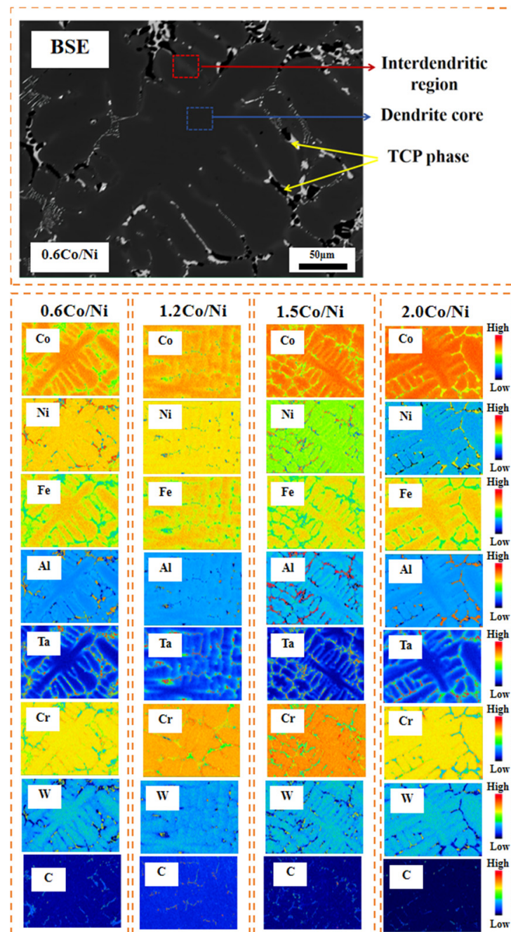
Figure 4. Element distribution in alloys with varying Co/Ni ratios. The enlarged BSE image of the 0.6Co/Ni alloy identifies key microstructural regions.
