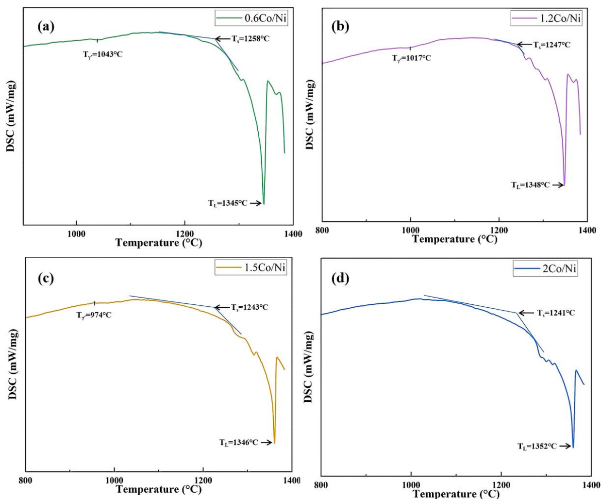
Figure 1. DSC heating curves and characteristic phase transition temperatures of alloys with different Co/Ni ratios: (a) 0.6Co/Ni; (b) 1.2Co/Ni; (c) 1.5Co/Ni; (d) 2.0Co/Ni.
