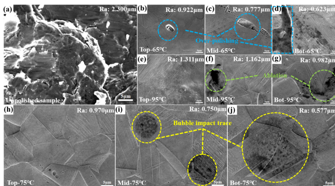
Figure 5. Surface morphology of the middle part of each micro-region before and after polishing under different temperature fields: (a)—Original sample; (b–d)—65 °C; (h–j)—75 °C; (e–g)—95 °C.
