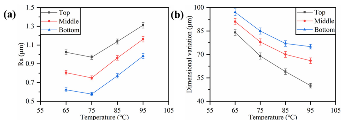
Figure 4. Roughness (a) and dimensional variation (b) in the middle of each micro-region after polishing under different temperature fields.
