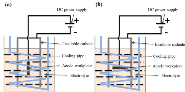
Figure 1. PEP device and sample placement of anode diagram: (a)—vertical placement; (b)—horizontal placement.
