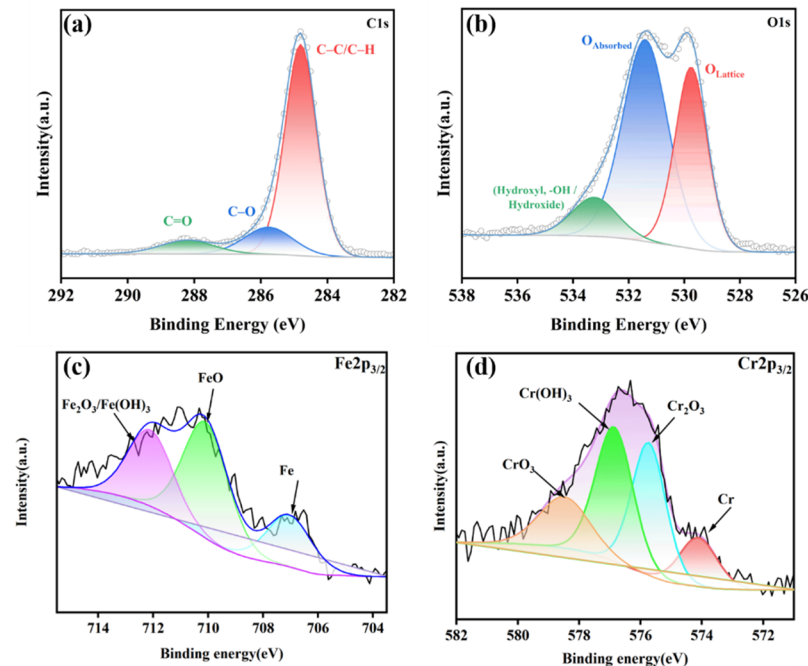
Figure 7. High-resolution XPS spectra of various elements after plasma electrolytic polishing: (a) C 1s, (b) O 1s, (c) Fe2p 3/2 , (d) Cr2p 3/2 .
