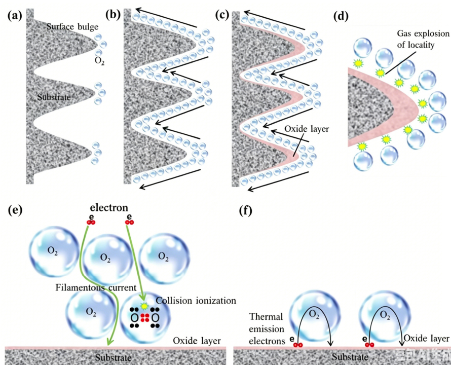
Figure 8. Model of PEP process: (a)—point effect; (b)—extended surface discharge; (c)—oxidized-sparse layer; (d)—gas explosion of locality; (e)—filamentary current and collision ionization; (f)—thermal electron emission.
