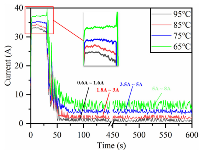
Figure 3. Curve of current variation during low-high stage polishing (50 V–30 s, 240 V–570 s) under various temperature fields.
