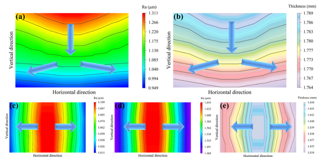
Figure 2. The surface roughness (a) and remaining thickness (b) of the entire specimen after polishing in vertical placement and the upper surface roughness (c), lower surface roughness (d) and remaining thickness (e) after polishing in horizontal placement.
