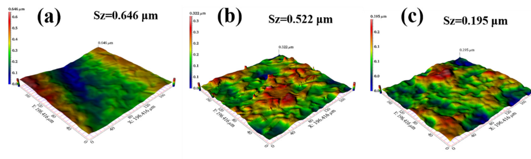
Figure 6. Three-dimensional profilometry images of different regions at 75 °C: (a) upper region, (b) middle region, (c) bottom region.
