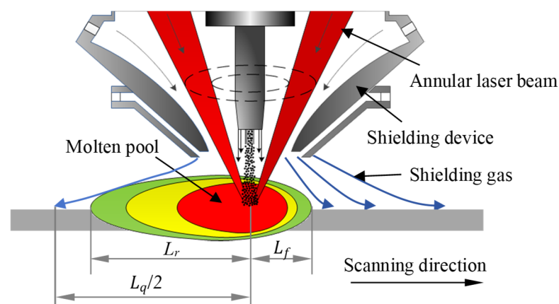
Figure 1. Schematic diagram of high-temperature area of melt pool and effective protection area.
