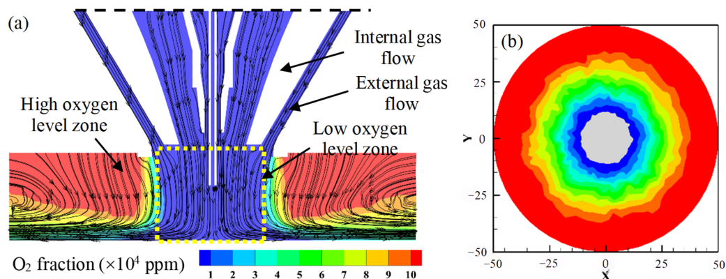
Figure 2. Oxygen content distribution: (a) longitudinal section; (b) transverse section.
