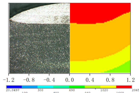
Figure 8. Comparison chart between simulation and experimental results of the molten pool.
