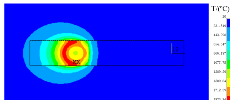
Figure 7. Temperature field of melt pool.
