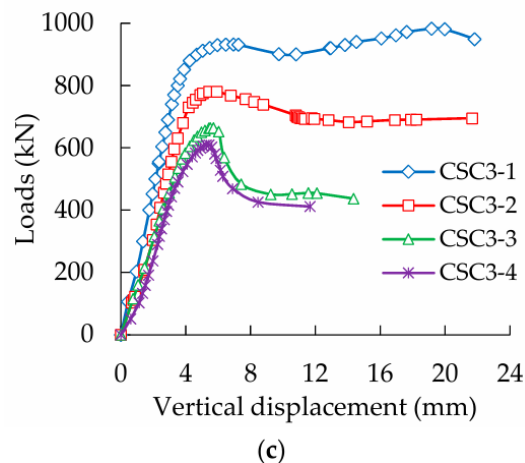
Figure 4. Load–vertical displacement behavior of CFST specimens with different corrosion ratios. (a) t = 0.92 mm; (b) t = 1.42 mm; (c) t = 1.92 mm [57].
