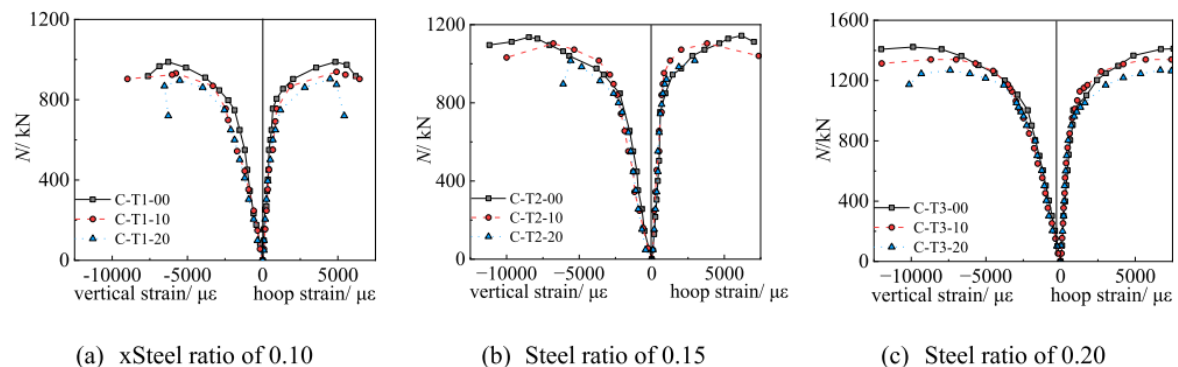
Figure 6. Axial load–strain curves of stub CFST columns [2].
