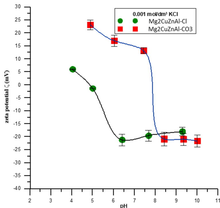
Figure 6. Zeta potential ( \zeta ) vs. pH for Mg 2 CuZnAl-Cl and Mg 2 CuZnAl-CO 3 measured in 0.001 mol/L KCl.
