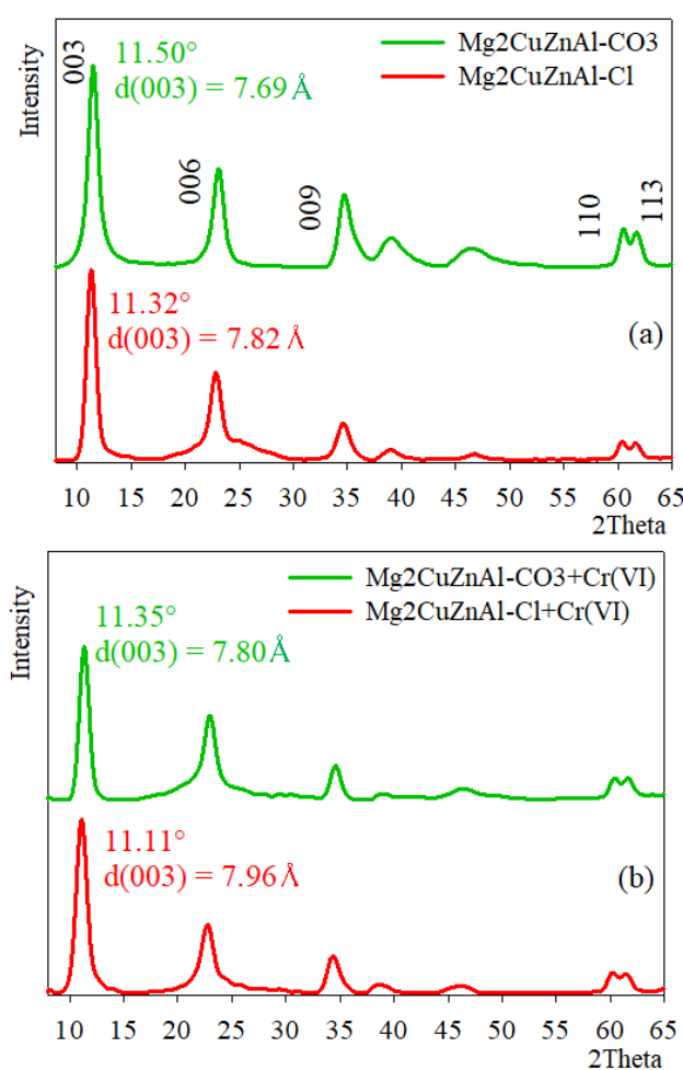
Figure 9. Powder XRD patterns of \text{Mg}_2\text{CuZnAl-CO}_3 and \text{Mg}_2\text{CuZnAl-Cl} sorbents before (a) and after (b) \text{Cr(VI)} sorption process.
