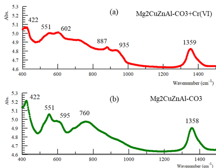
Figure 10. FTIR spectra of \text{Mg}_2\text{CuZnAl-CO}_3 with adsorbed chromate anions (a) and \text{Mg}_2\text{CuZnAl-CO}_3 (b).
