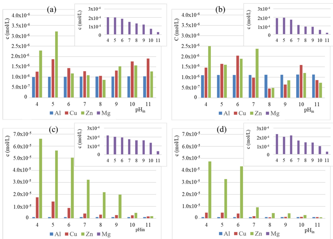
Figure 8. Stability of the LDH structure depending on pH: Mg 2 CuZnAl-CO 3 (a), Mg 2 CuZnAl-CO 3 + Cr(VI) (b), Mg 2 CuZnAl-Cl (c), Mg 2 CuZnAl-Cl + Cr(VI) (d).
