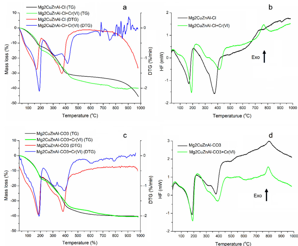
Figure 11. TG-DTG (a,c) and DSC (b,d) curves of Mg 2 CuZnAl-CO 3 , Mg 2 CuZnAl-CO 3 + Cr(VI), Mg 2 CuZnAl-Cl, and Mg 2 CuZnAl-Cl + Cr(VI) recorded in air atmosphere.
