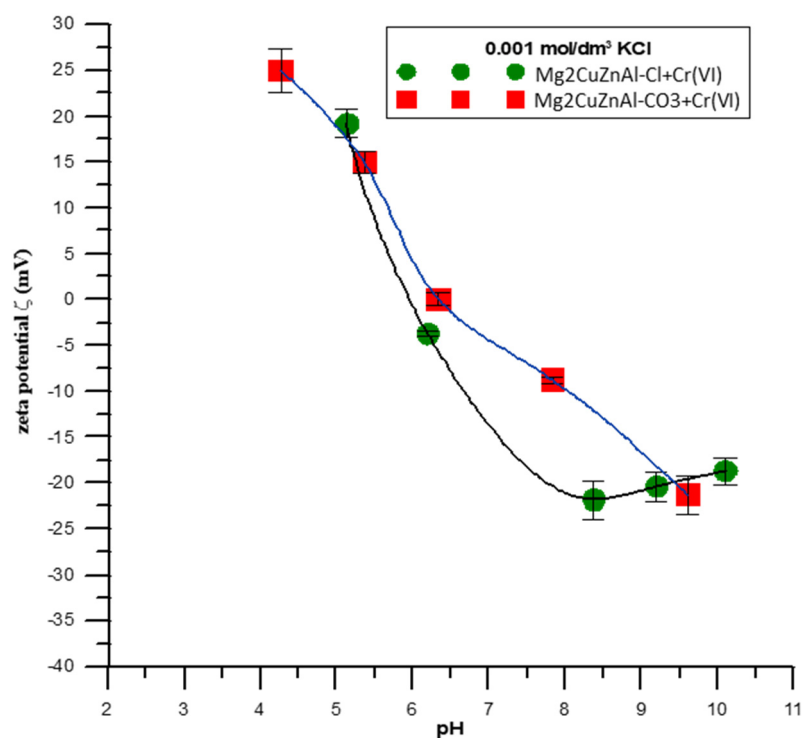
Figure 7. Zeta potential ( \zeta ) vs. pH for Mg 2 CuZnAl-Cl and Mg 2 CuZnAl-CO 3 after Cr(VI) sorption process measured in 0.001 mol/L KCl.
