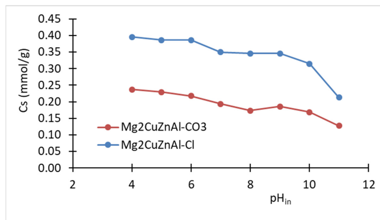
Figure 5. Changes in the sorption quantity on \text{Mg}_2\text{CuZnAl-Cl} and \text{Mg}_2\text{CuZnAl-CO}_3 forms depending on the pH of the initial \text{Cr(VI)} solution.
