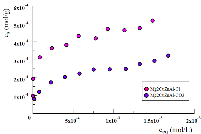
Figure 3. Changes in the sorption quantity on Mg 2 CuZnAl-Cl and Mg 2 CuZnAl-CO 3 forms depending on the equilibrium concentration of Cr(VI).
