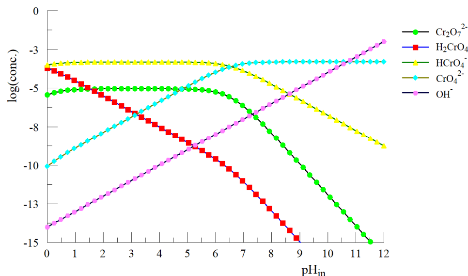
Figure 4. Speciation of chromium(VI) ions in aqueous solutions depending on pH ( [\text{Cr(VI)}]_t = 0.5 \text{ mmol/L} ).
