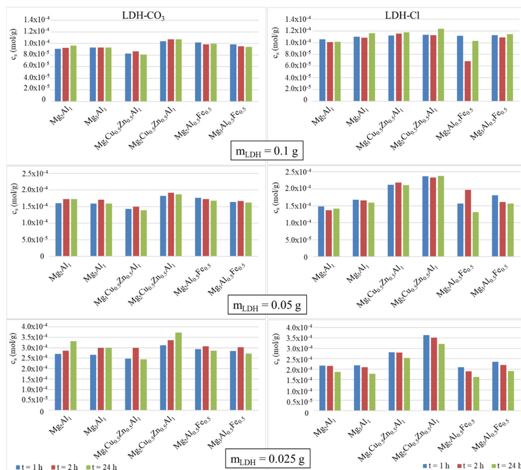
Figure 2. Comparison of the efficiency of the \text{Cr(VI)} anion sorption process on all synthesized LDH materials, both in chloride and carbonate form; c_{in} = 0.5 \text{ mmol/L} , V = 25 \text{ mL} , \text{pH} = 7.2 , t = 1, 2, 24 \text{ h} , and the mass of the adsorbent used ( m = 0.025, 0.05, 0.1 \text{ g} ).
