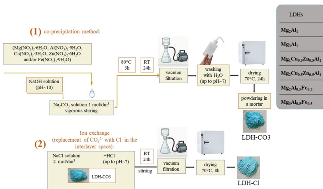
Figure 1. Schematic diagram showing the main steps of LDH synthesis by the co-precipitation method, leading to the formation of chloride- and carbonate-intercalated LDHs. (Photographs of powdered LDH-Cl and LDH-CO 3 are shown for Mg 2 Cu 0.5 Zn 0.5 Al 1 -Cl and Mg 2 Cu 0.5 Zn 0.5 Al 1 -CO 3 as representative examples).
