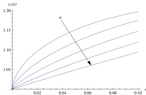
Figure 4. The approximate solution for \alpha = 0.6, 0.7, 0.8, 0.9, 1 .
