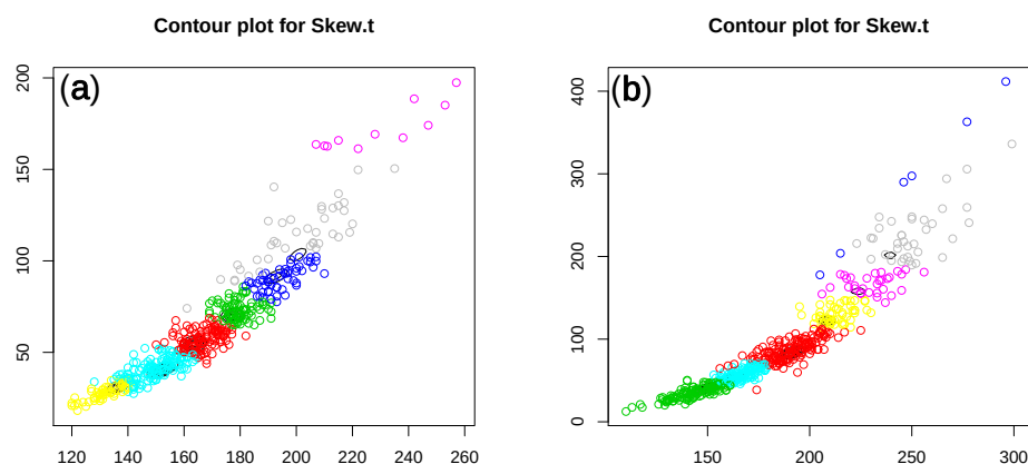
Figure 3. Selected FMST fits for (a) males ( m = 6 ) and (b) females ( m = 7 ). Each color is related to each FMST component.
