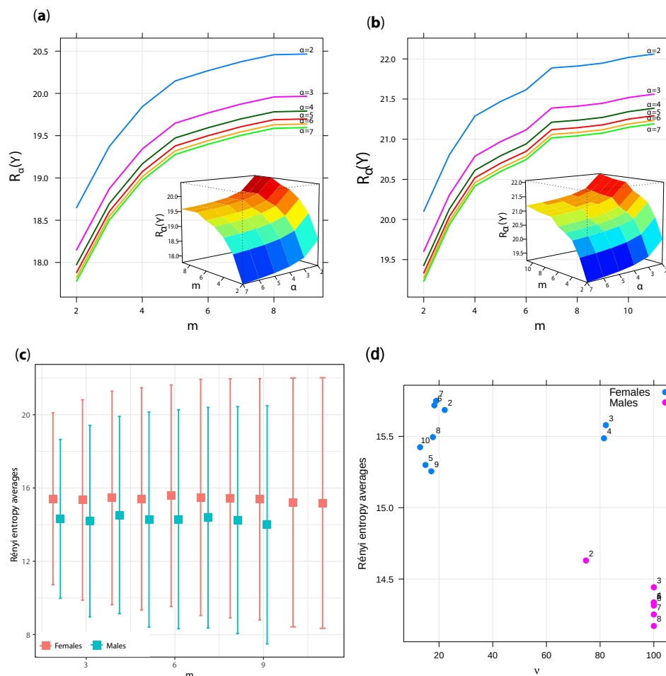
Figure 2. Upper bounds for Rényi entropies based on finite mixture of skew- t (FMST) distribution [R_\alpha(\mathbf{Y})] by number of components ( m ), for (a) males and (b) females, respectively. 3d-subplots correspond to R_\alpha(\mathbf{Y}) versus m and \alpha . Panel (c) shows the whisker plots of lower and upper bounds for Rényi entropies based on FMST distribution, and their respective averages by gender and number of components m . Panel (d) shows a dispersion plot between R_\alpha(\mathbf{Y}) and \nu by gender, where the number of each point corresponds to m .
