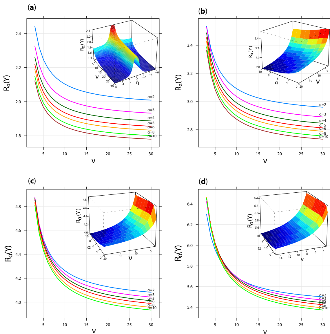
Figure 1. Skew- t Rényi entropy [R_\alpha(\mathbf{Y})] versus degree of freedom parameter ( \nu = 3, \dots, 30 ) for cases (a–d) described above. Each line corresponds to order \alpha = 2, 3, 4, 5, 6, 8, 10 . 3d-subplot of case (a) corresponds to R_\alpha(\mathbf{Y}) versus \nu and \eta , whereas the 3d-subplots of cases (b–d) are R_\alpha(\mathbf{Y}) versus \nu and \alpha .
