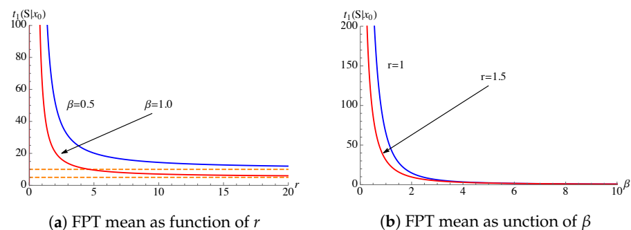
Figure 5. The FPT mean (54) is plotted for x_0 = 5 , S = 10 and \alpha = -0.5 . The dashed lines in (a) indicate the asymptotic limit (S - x_0)/\beta .
