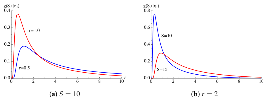
Figure 3. The FPT pdf (32) is plotted as function of t for t_0 = 0 , x_0 = 5 .
