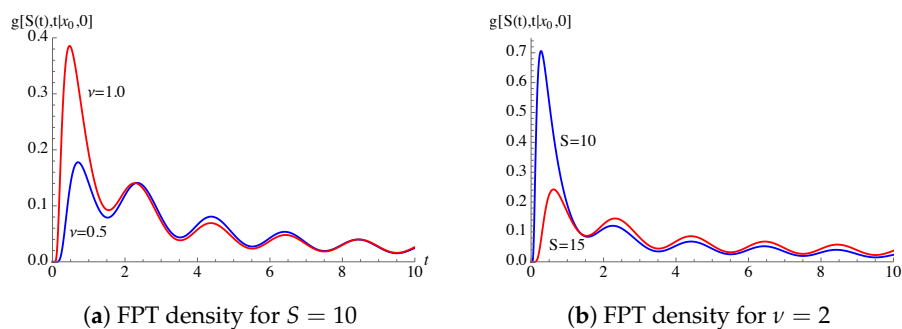
Figure 6. For the Feller-type process having B_1(x, t) = -0.05x + r(t)/2 and B_2(x, t) = 2r(t)x , with r(t) = v[1 + 0.4 \sin(\pi t)] , the FPT pdf (83) from x_0 = 5 through S(t) = S e^{\alpha t} is plotted as a function of t .
