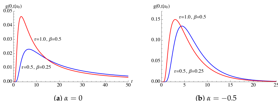
Figure 1. The FPT pdf (23) is plotted as function of t for t_0 = 0 , x_0 = 5 .
