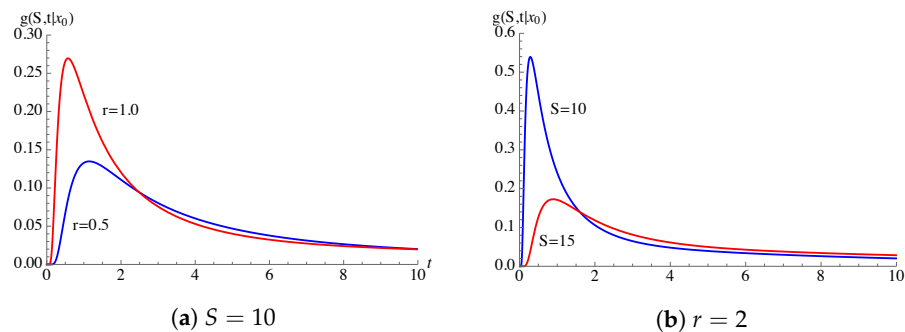
Figure 2. The FPT pdf (28) is plotted as function of t for t_0 = 0 and x_0 = 5 .
