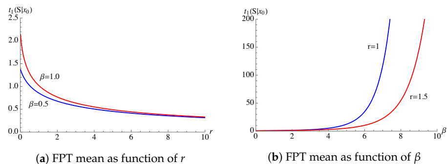
Figure 4. The FPT mean (54) is plotted for x_0 = 5 , S = 3 and \alpha = -0.5 .
