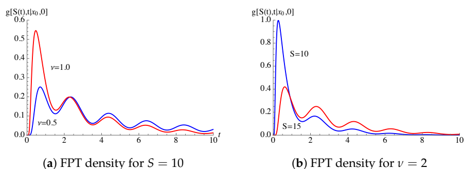
Figure 7. For the Feller-type process, having B_1(x, t) = -0.05x + 3r(t)/2 and B_2(x, t) = 2r(t)x , with r(t) = \nu[1 + 0.4\sin(\pi t)] , the FPT pdf (88) from x_0 = 5 through S(t) = S e^{\alpha t} is plotted as function of t .
