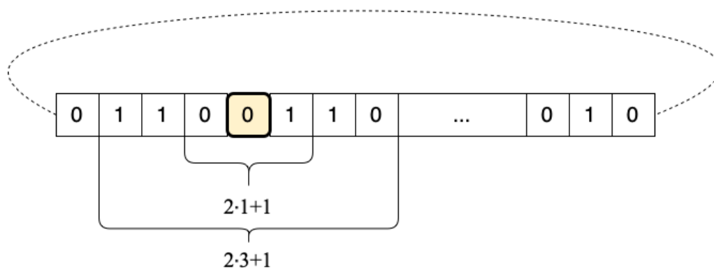
Figure 3. Neighborhoods containing 2r + 1 cells, r = 1 and r = 3 .
