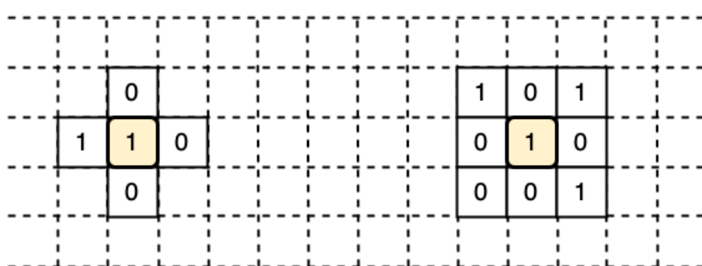
Figure 4. (Left): von Neuman neighborhood; (Right): Moore neighborhood.
