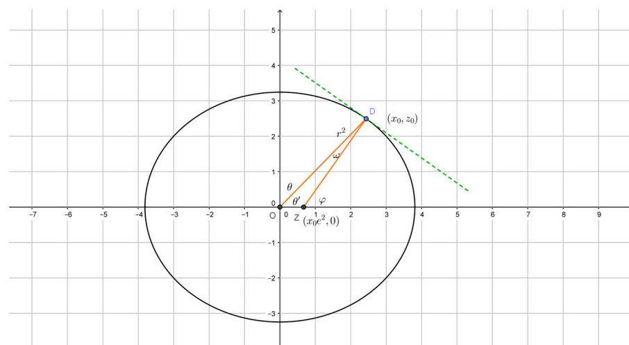
Figure 1. Let \gamma be an ellipse with semimajor axis a and semiminor axis b .
