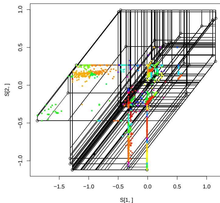
Figure 4. The tropical polytope of gene trees for the housekeeping genes. Black points in the figures are outliers found by the tropical KDE. In order to visualize this, we apply the tropical PCA. Each color represents an unique tree topology.
