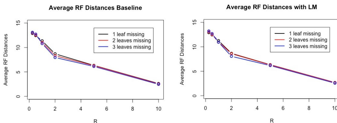
Figure 3. This figure shows performance on the baseline model (left) and linear regression models (Right). For each category, we infer 200 trees from 800 trees. The x-axis represents the ratio R and the y-axis shows the average Robinson–Foulds distances between estimated trees and true trees for 200 trees. The smaller the Robinson–Foulds distance is, the better the performance. As one can see, these results are very close to each other for all R .
