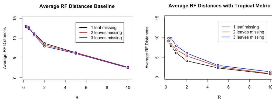
Figure 2. This figure shows performance on the baseline (Left) and our method using a tropical polytope (Right). For each category, we infer 200 trees from 800 trees. The x-axis represents the ratio R and the y-axis shows the average Robinson–Foulds distances between estimated trees and true trees for 200 trees. The smaller the Robinson–Foulds distance is, the better the performance.
