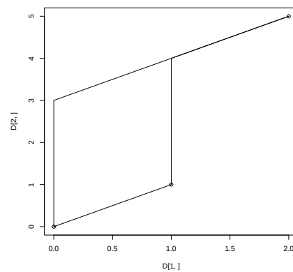
Figure 1. Tropical polytope of three points (0, 0, 0), (0, 1, 1), (0, 2, 5) \in \mathbb{R}^3/\mathbb{R}\mathbf{1} .
