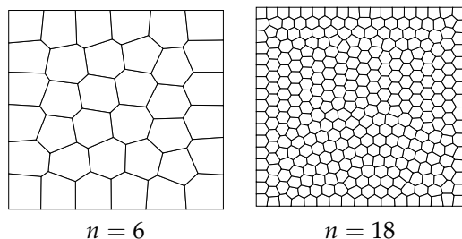
Figure 8. Meshes with 6 \times 6 and 18 \times 18 elements.
