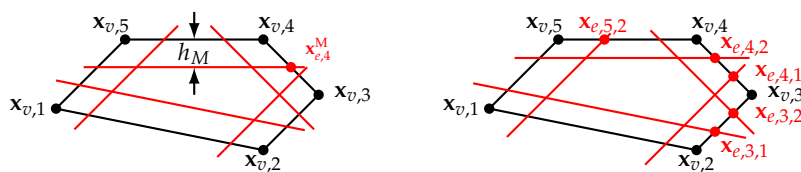
Figure 6. The two sub-partitions of E_5 used for constructing specific H^p supplemental functions. The left one is used for \mathcal{DS}_r^M and \mathbf{V}_r^{M,s} , where h_M = \lambda_5(x_{e,4}^M) . The right one is used for \mathcal{DS}_r^T and \mathbf{V}_r^{T,s} , where the closest trisection points are marked in red.
