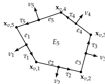
Figure 1. A pentagon E_5 , with edges e_i , outer unit normals v_i , tangents \tau_i , and vertices x_{v,i} .
