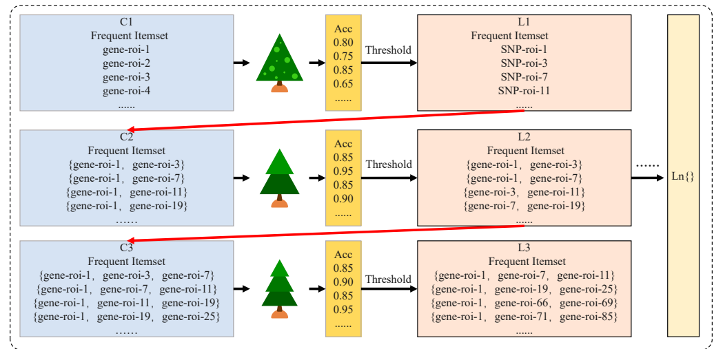
Figure 3. The steps of the decision tree–Apriori model.
