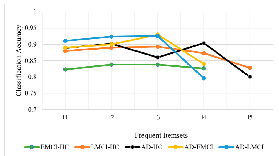
Figure 5. The accuracy of leave-one-out cross-validation of the test set of all frequent itemsets in 5 datasets.
