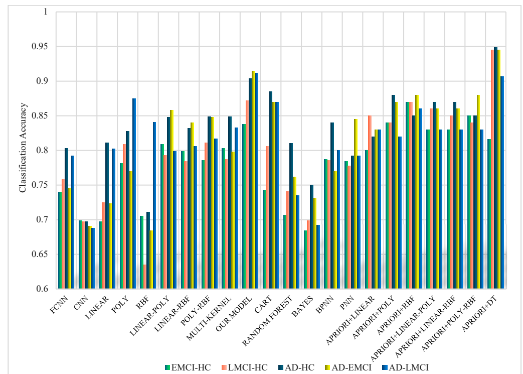
Figure 9. The comparison with other methods in 5 datasets. DT = Decision Tree; PNN = Product-based Neural Network; BPNN = Back-Propagation Neural Network; CART = Classification and Regression Tree; CNN = Convolutional Neural Network; FCNN = Fully Connected Neural Network.
