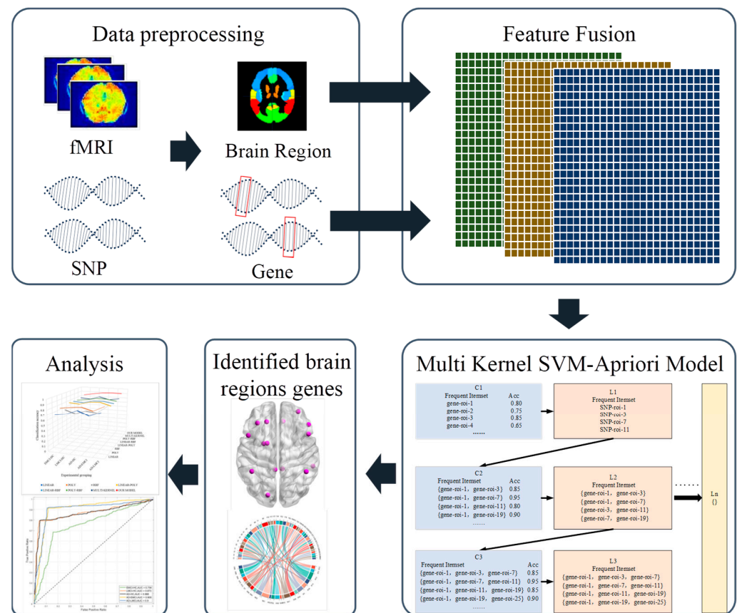
Figure 1. The framework of Multi Kernel SVM–Apriori Model analysis.
