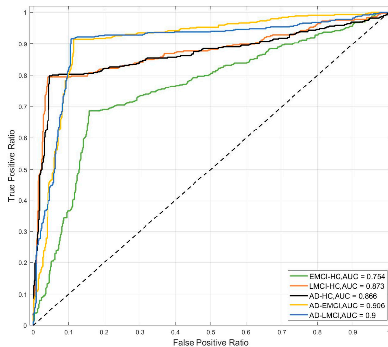
Figure 8. The ROC curve of the best accuracy in each dataset. The dashed line represents the performance of a random classifier.
