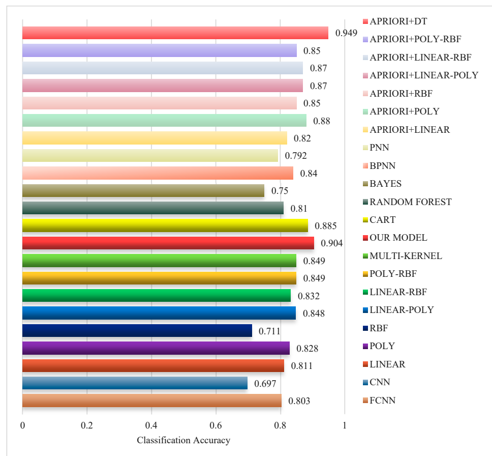
Figure 7. The comparison with other methods in S_{AD\_HC} . DT = Decision Tree; PNN = Product-based Neural Network; BPNN = Back-Propagation Neural Network; CART = Classification and Regression Tree; CNN = Convolutional Neural Network; FCNN = Fully Connected Neural Network.
