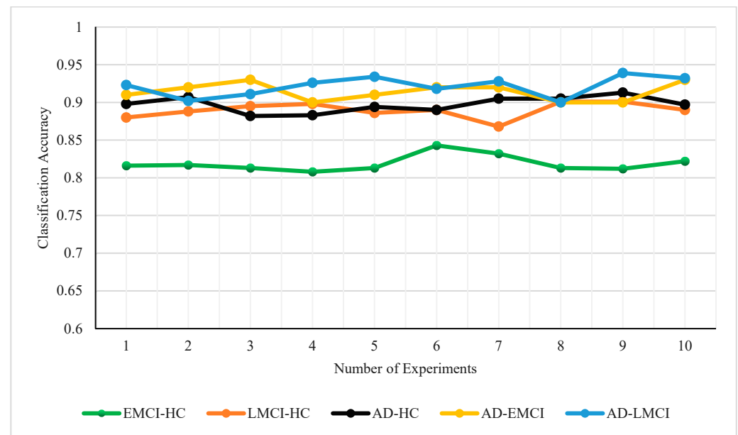
Figure 10. The 10 independent validation experiments accuracy of leave-one-out cross-validation of the test set in 5 datasets. HC = Healthy Control; EMCI = Early Mild Cognitive Impairment; LMCI = Late Mild Cognitive Impairment; AD = Alzheimer’s Disease.
