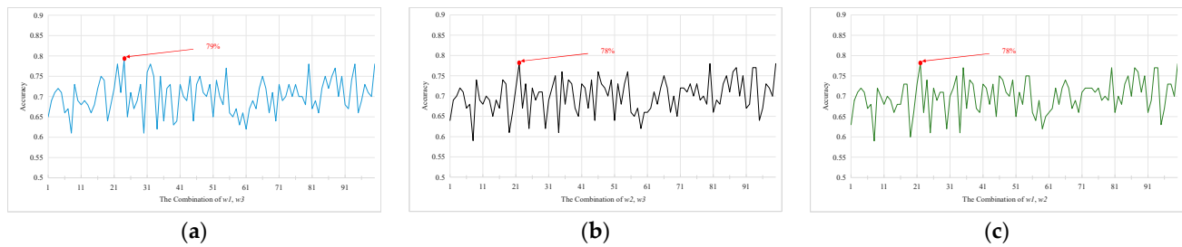
Figure 6. The curve of weight selection of dual-kernel SVM in S_{AD\_HC} . (a) The combination of w_1, w_3 and their accuracy in S_{AD\_HC} . (b) The combination of w_2, w_3 and their accuracy in S_{AD\_HC} . (c) The combination of w_1, w_2 and their accuracy in S_{AD\_HC} .
