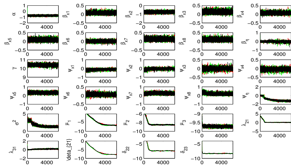
Figure 5. Trace plots of the estimates of unknown parameters against the number of iterations under SS prior, in which the colored solid lines represent the traces of estimates under three starting values: CHFS data.
