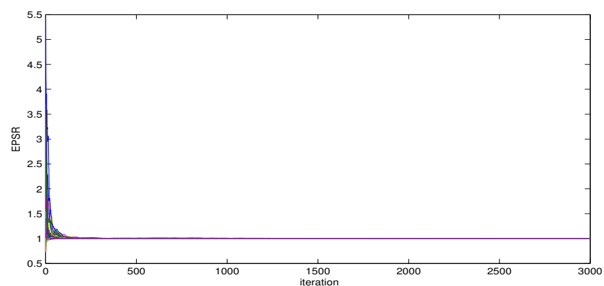
Figure 2. Plot of the values of EPSR of unknown parameters under three different starting values in which the colored solid lines represent the trajectories of EPSR of estimates against the number of iterations: simulation study and n = 400 .
