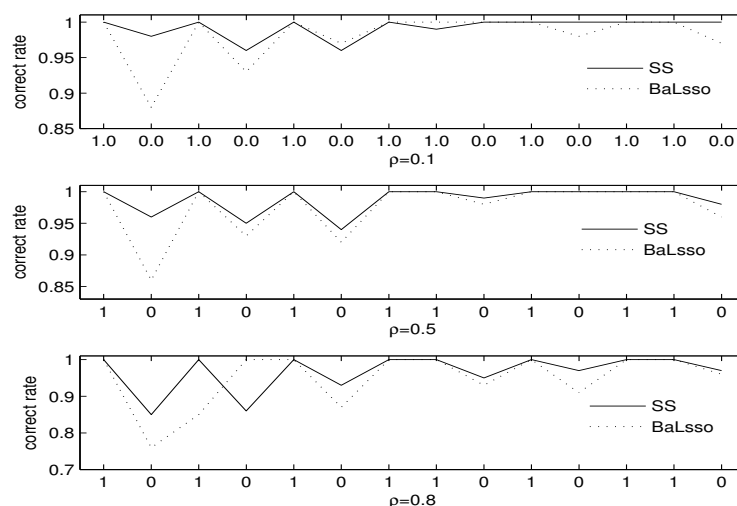
Figure 3. Plots of the correct rates of the selected variables under three scenarios: simulation study and n = 1000 .
