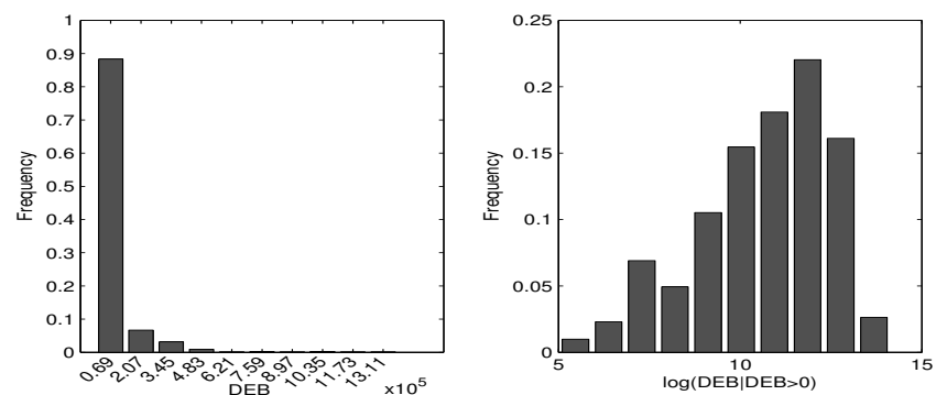
Figure 4. Histograms of DEB and the logarithms of their positive values: Chinese Household Financial Survey data. Left panel corresponds to DEB and right panel corresponds to \log(\text{DEB}|\text{DEB} > 0) .
