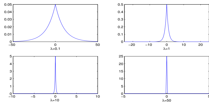
Figure 1. Plot of the densities of Laplace distribution for different choices of \lambda .
