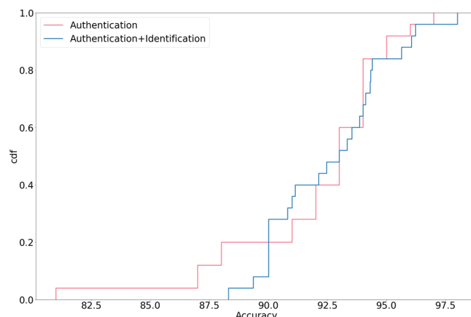
Figure 13. Cumulative distributive plot of accuracy.
