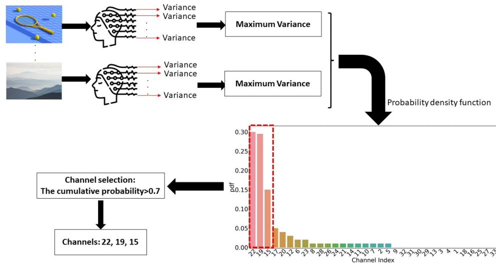
Figure 2. The flowchart of channel selection algorithm.
