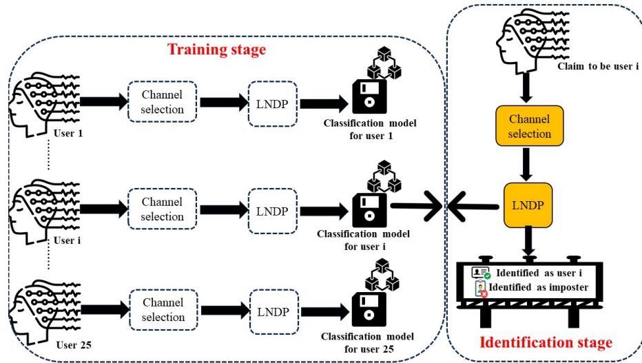
Figure 6. The identification stage pipeline.
