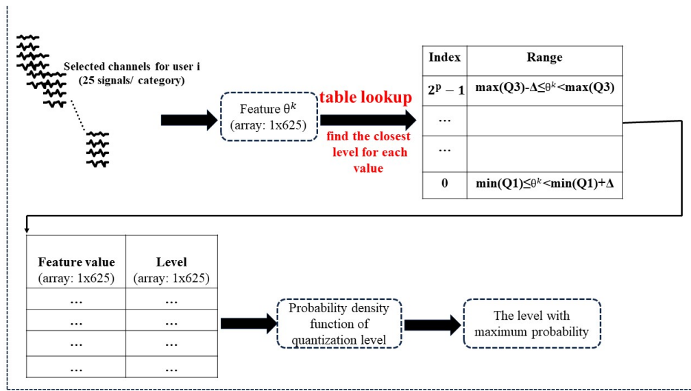
Figure 4. The flowchart of password generation algorithm.
