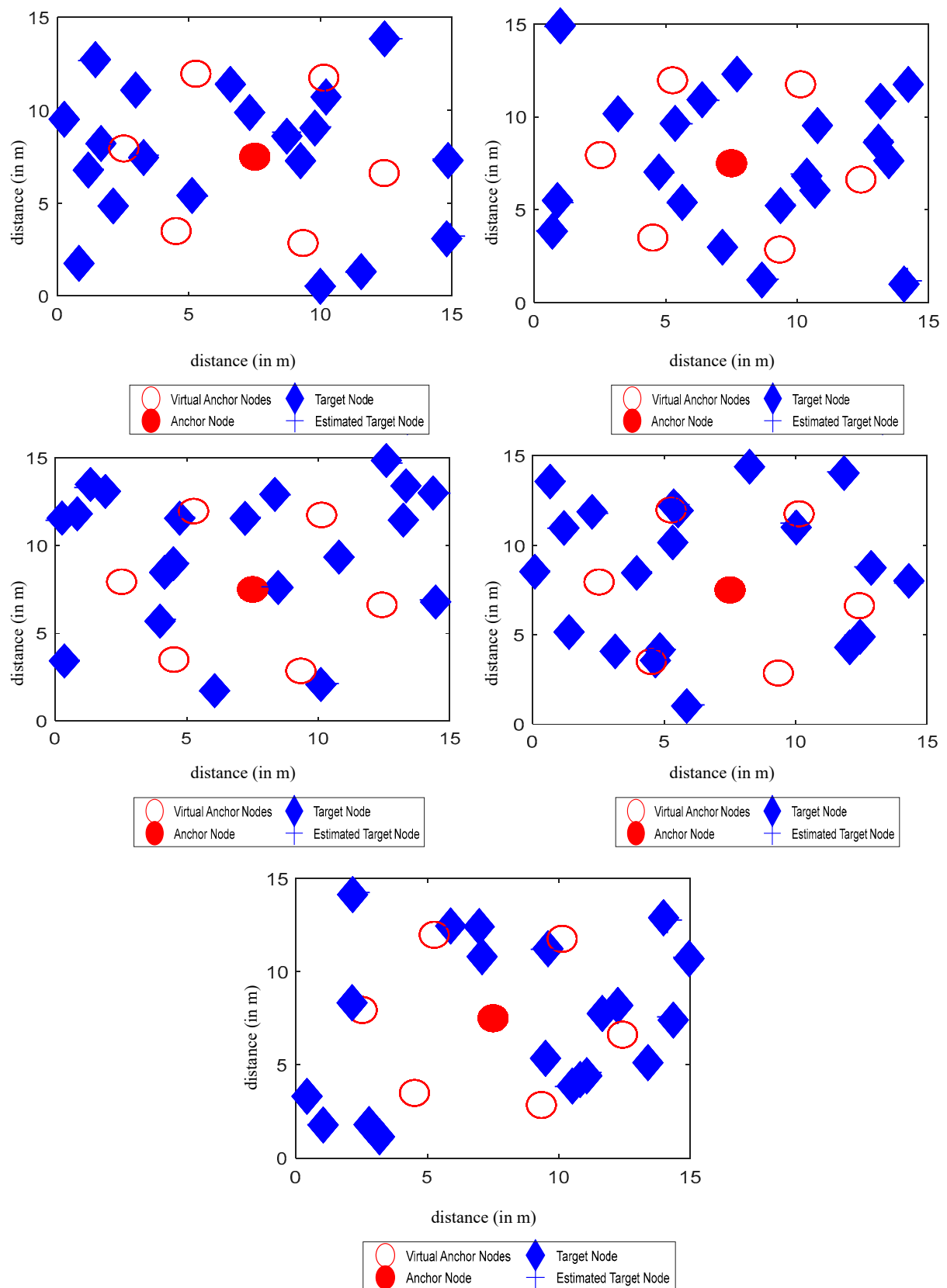
Figure 13. Node localization using WONMRA.
