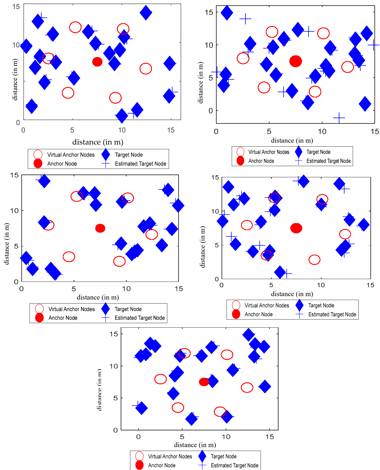
Figure 11. Node localization using NMRA.
