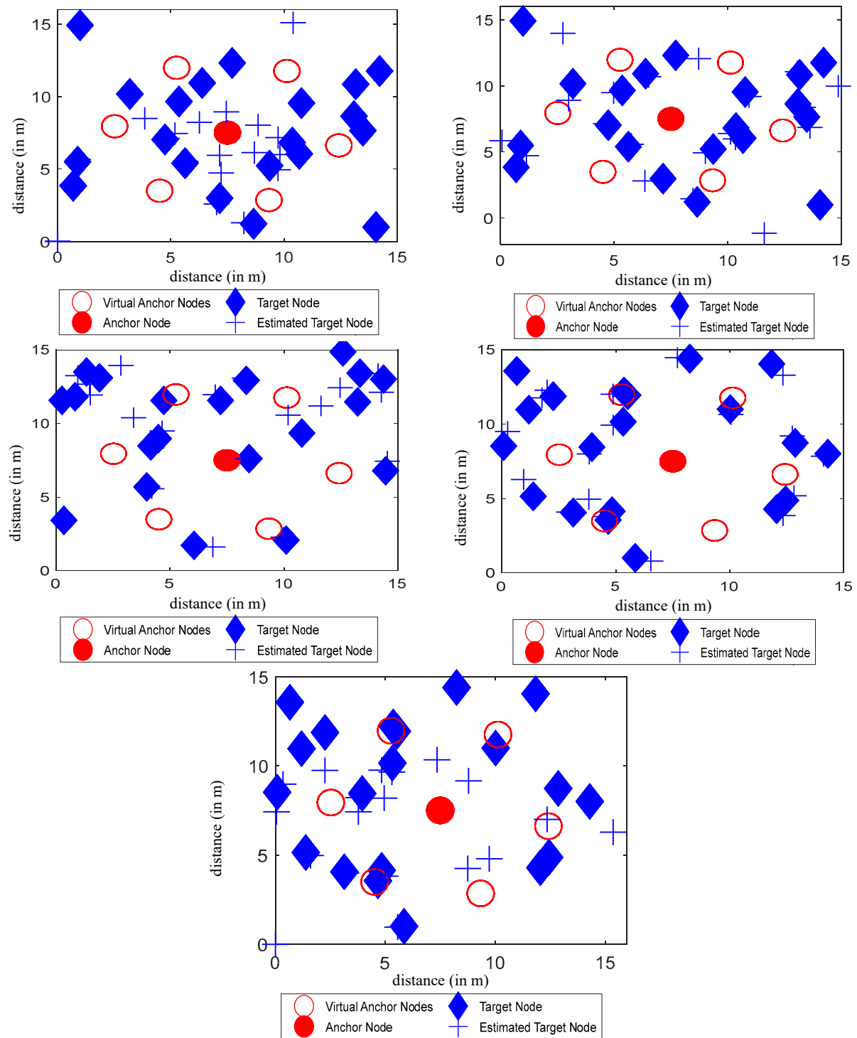
Figure 12. Node localization using WOA.
