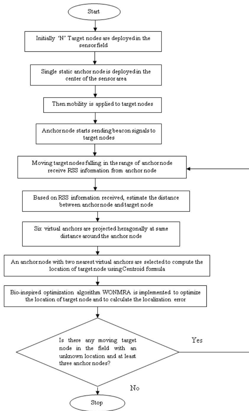
Figure 2. Process of localization.
