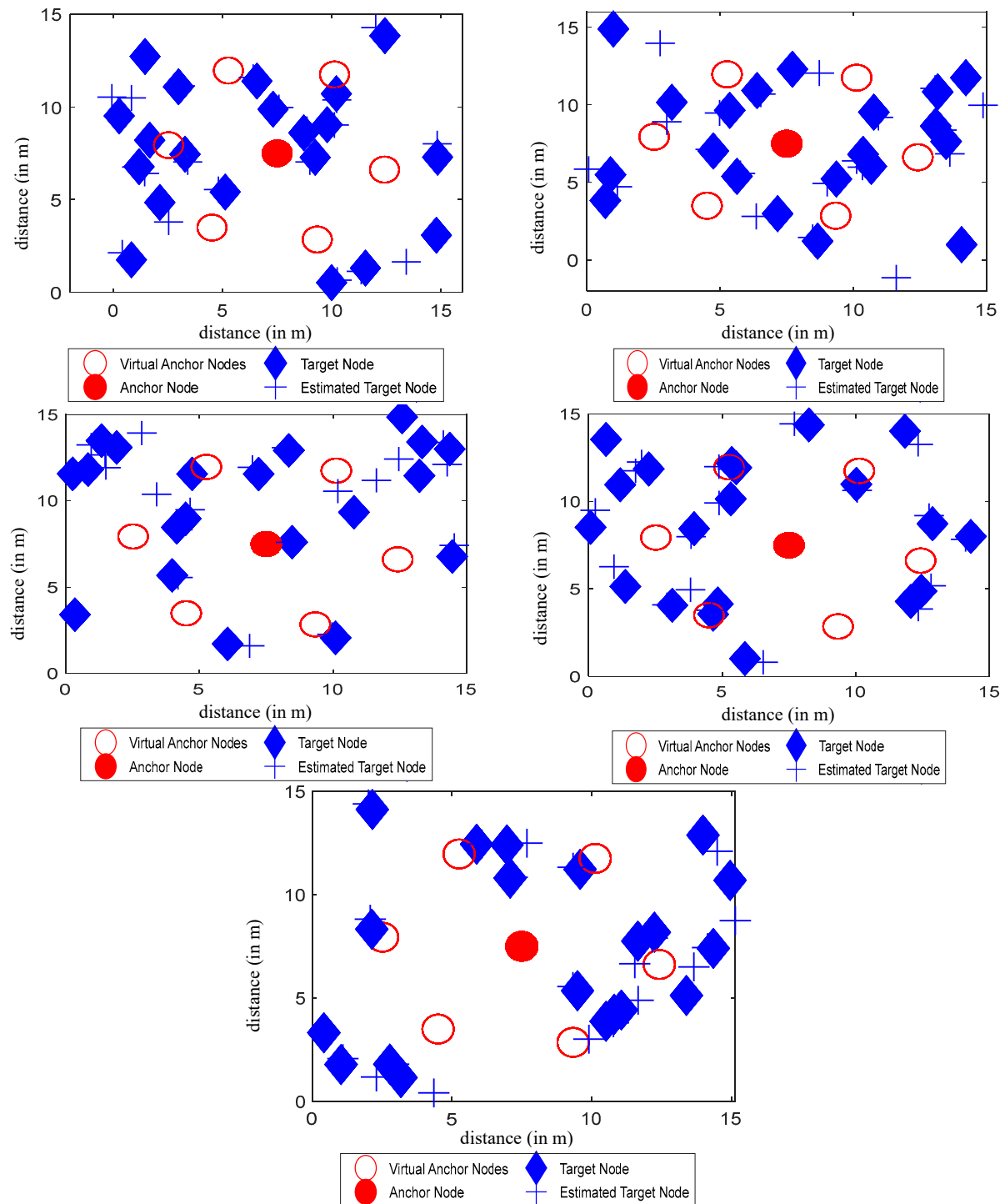
Figure 8. Node localization using PSO.
