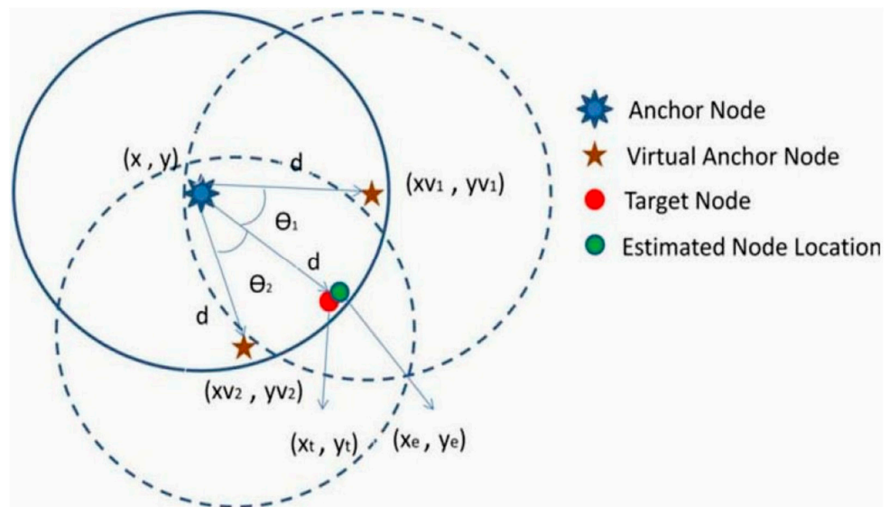
Figure 6. Error estimation using WONMRA.
