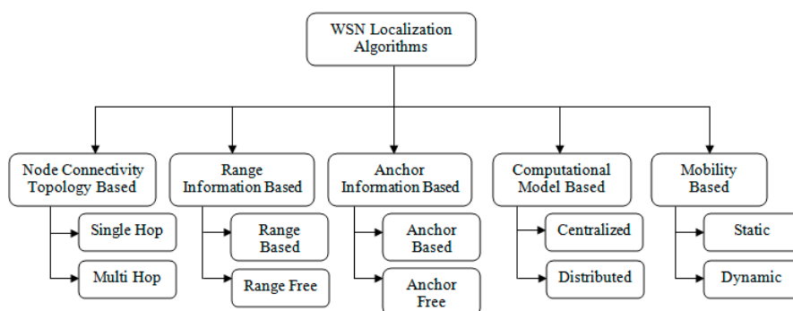
Figure 1. Localization algorithms.
