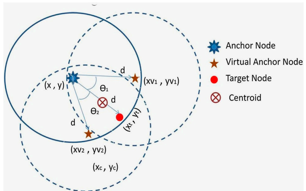
Figure 4. Centroid calculation.
