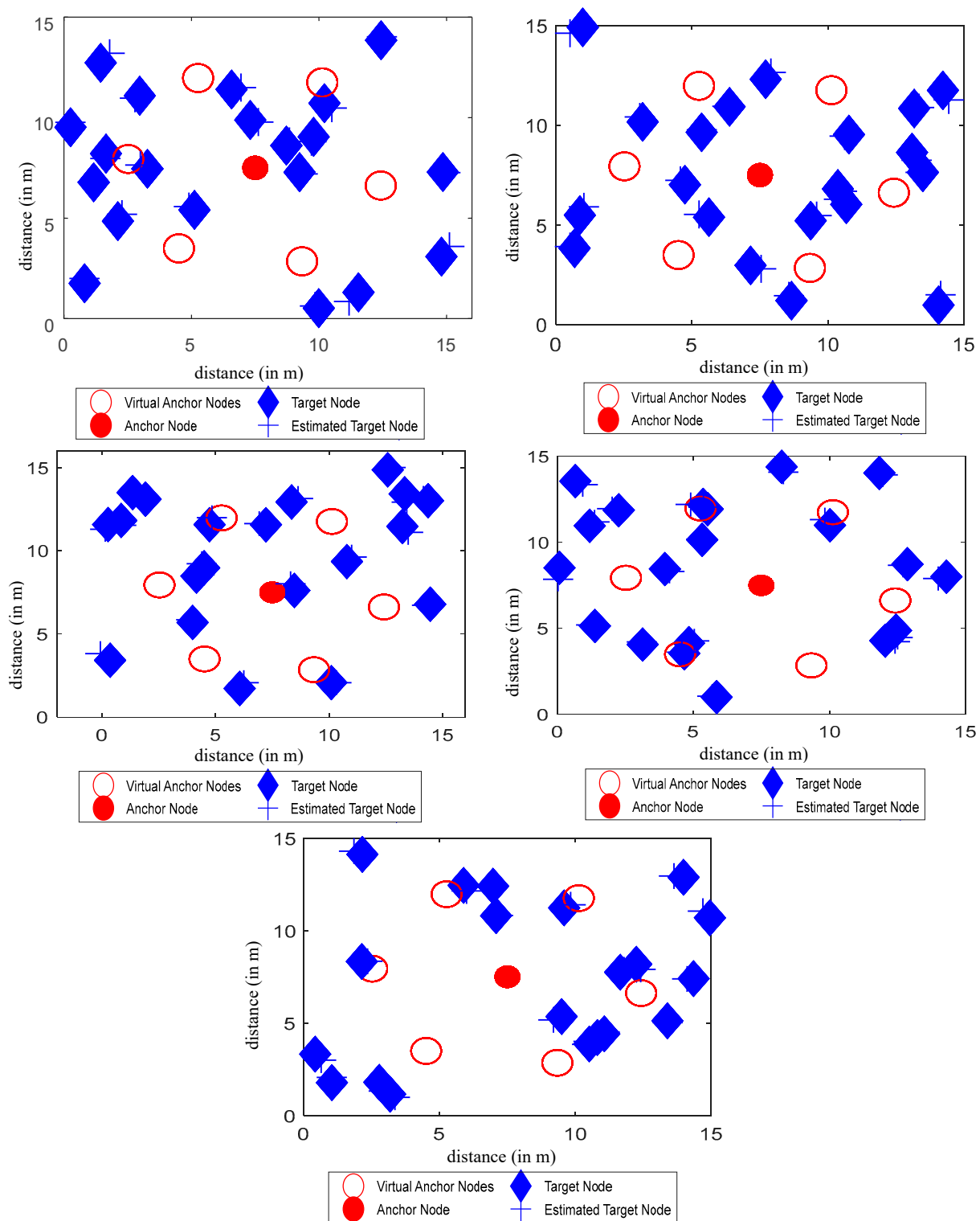
Figure 10. Node localization using HPSO.
