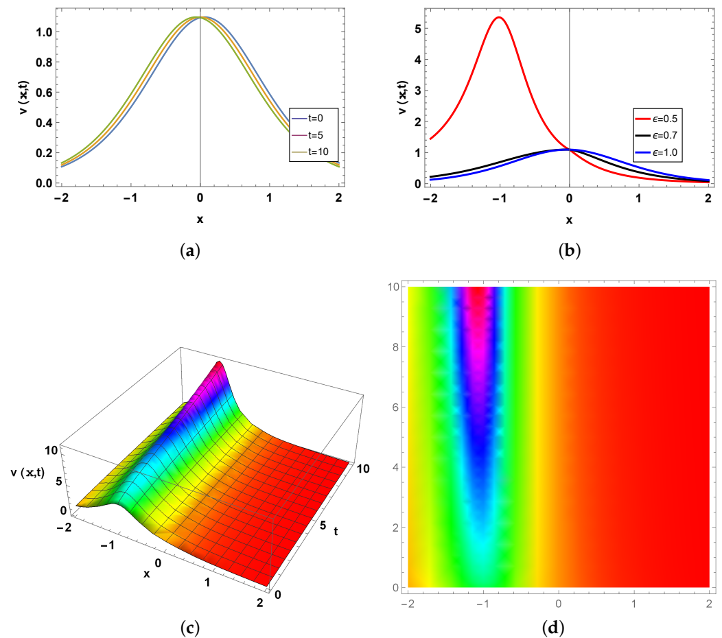
Figure 3. Plot for v(x,t) , as shown in Equation (32). (a) Two-dimensional graph for different values of t . (b) Two-dimensional graph for different values of \epsilon . (c) Three-dimensional graph for \epsilon = 0.6 . (d) Density graph for \epsilon = 0.6 .
