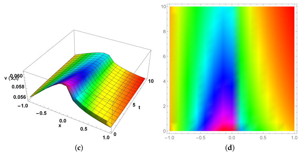
Figure 5. Plot for v(x, t) , as shown in Equation (44). (a) Two-dimensional plot for distinct values of t . (b) Two-dimensional graph for different values of \epsilon . (c) Three-dimensional graph for \epsilon = 0.6 . (d) Density graph for \epsilon = 0.6 .
