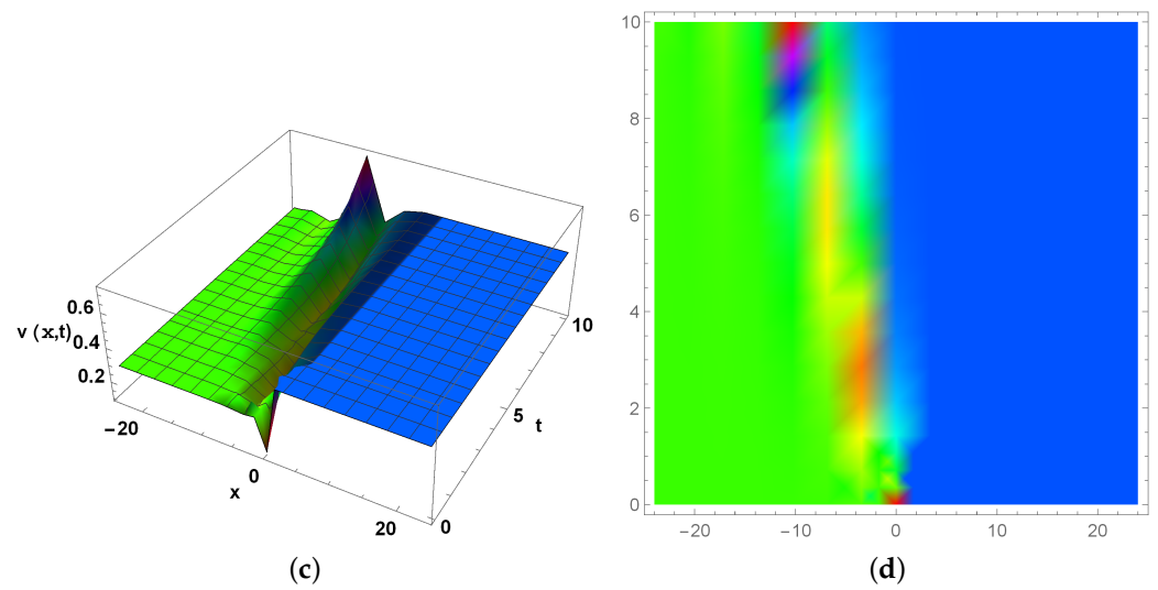
Figure 2. Plot for v(x,t) , as shown in Equation (20). (a) Two-dimensional plot for distinct values of t . (b) Two-dimensional graph for different values of \epsilon . (c) Three-dimensional graph for \epsilon = 0.6 . (d) Density graph for \epsilon = 0.6 .
