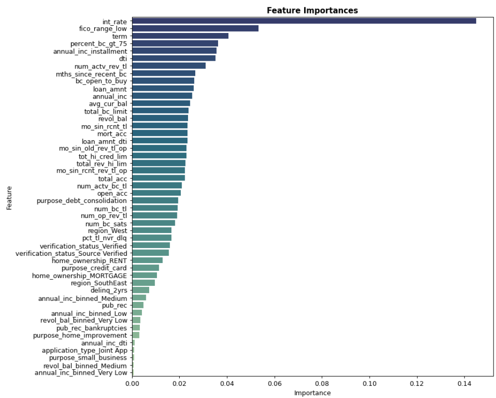
Figure 9. Feature importance.
