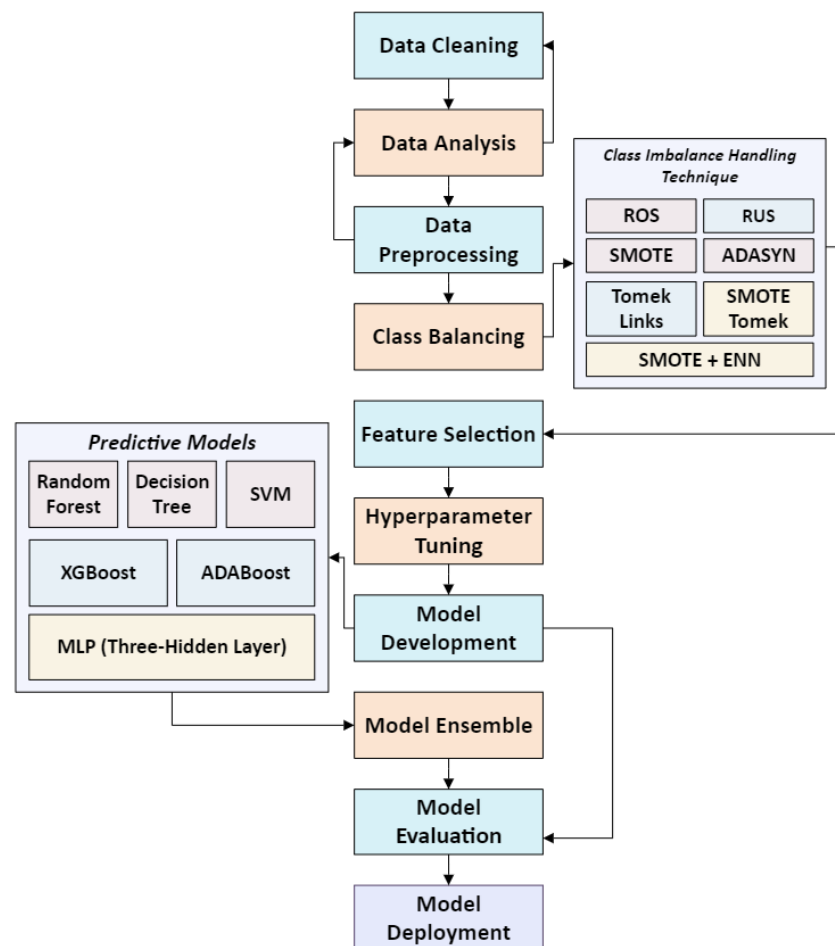
Figure 1. Research framework.
