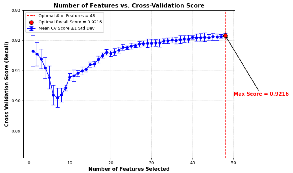
Figure 8. Features selected.
