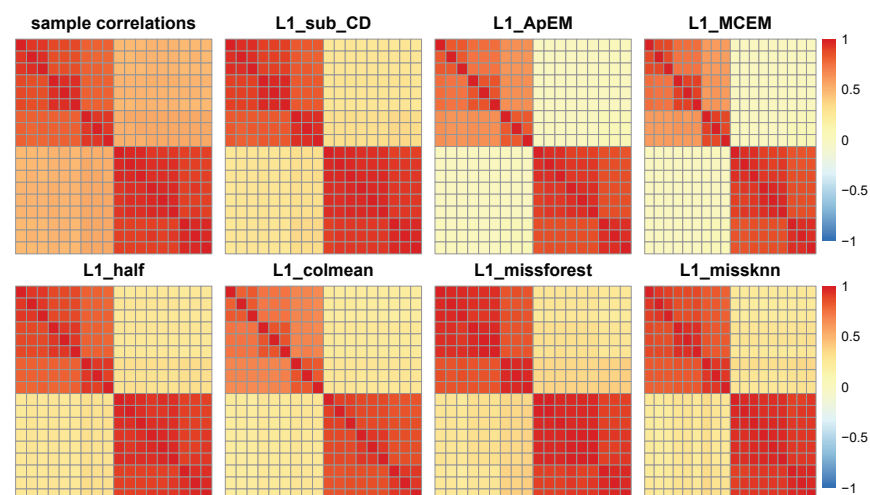
Figure 7. Heat maps of correlation coefficient matrices estimated by L1_ApEM, L1_MCEM, L1_missforest, L1_missknn, L1_half, L1_colmean, L1_sub_CD and sample correlations for proteomic dataset.
