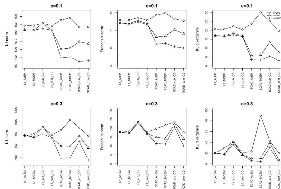
Figure 2. Line charts of average L_1 norm, Frobenius norm, KL divergence for cliques model with p = 100 under both L_1 and SCAD penalties.
