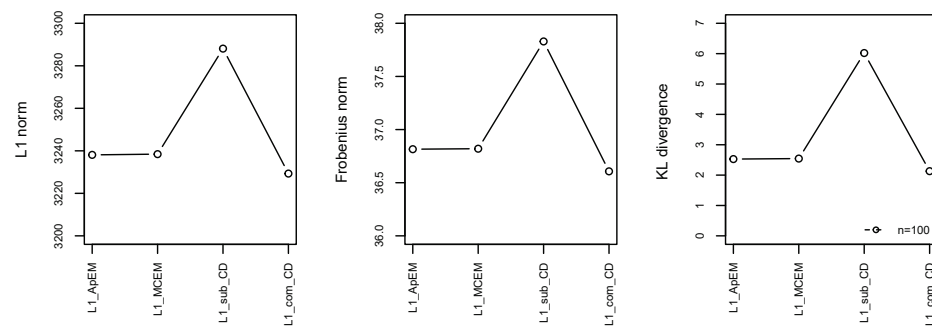
Figure 6. Line charts of average L_1 norm, Frobenius norm, KL divergence for cliques model with c = 0.1, p = 200, n = 100 under the L_1 penalty.
