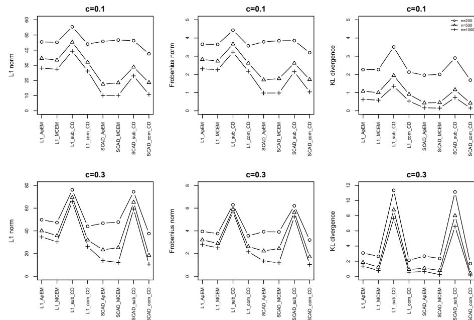
Figure 1. Line charts of average L_1 norm, Frobenius norm, KL divergence for cliques model with p = 30 under both L_1 and SCAD penalties.
