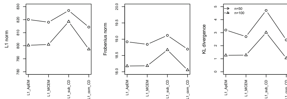
Figure 5. Line charts of average L_1 norm, Frobenius norm, KL divergence for the cliques model with c = 0.1, p = 100, n = 50, 100 under the L_1 penalty.
