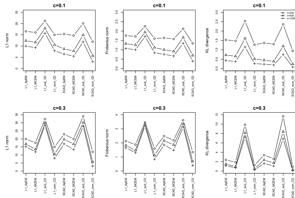
Figure 3. Line charts of average L_1 norm, Frobenius norm, KL divergence for the moving average model with p = 30 under both L_1 and SCAD penalties.
