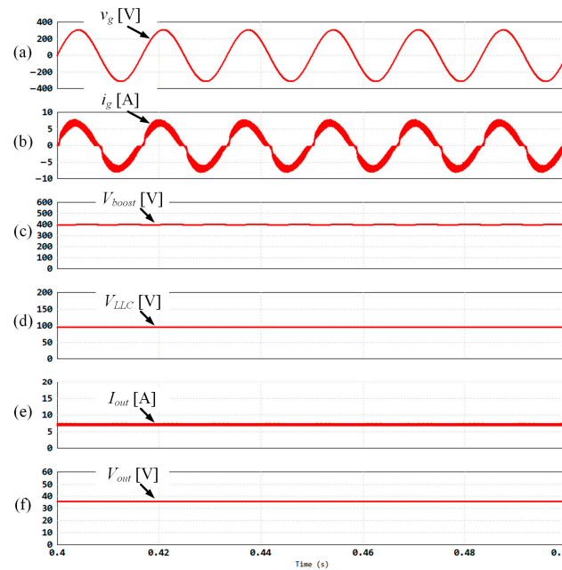
Figure 11. Various simulation results of the PMD battery charger: (a) Voltage of the single-phase grid; (b) current of the single-phase grid; (c) PFC boost converter output voltage; (d) half-bridge LLC resonant converter output voltage; (e) battery charger output current; (f) battery charger output voltage.
