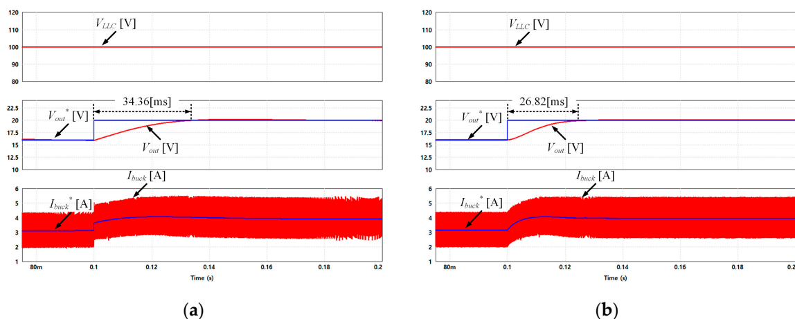
Figure 12. Simulation results of transient state responses: (a) PI controller; (b) proposed RBFLC.
