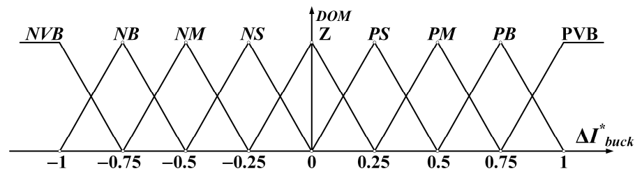
Figure 7. Membership function of \Delta I_{buck}^* .
