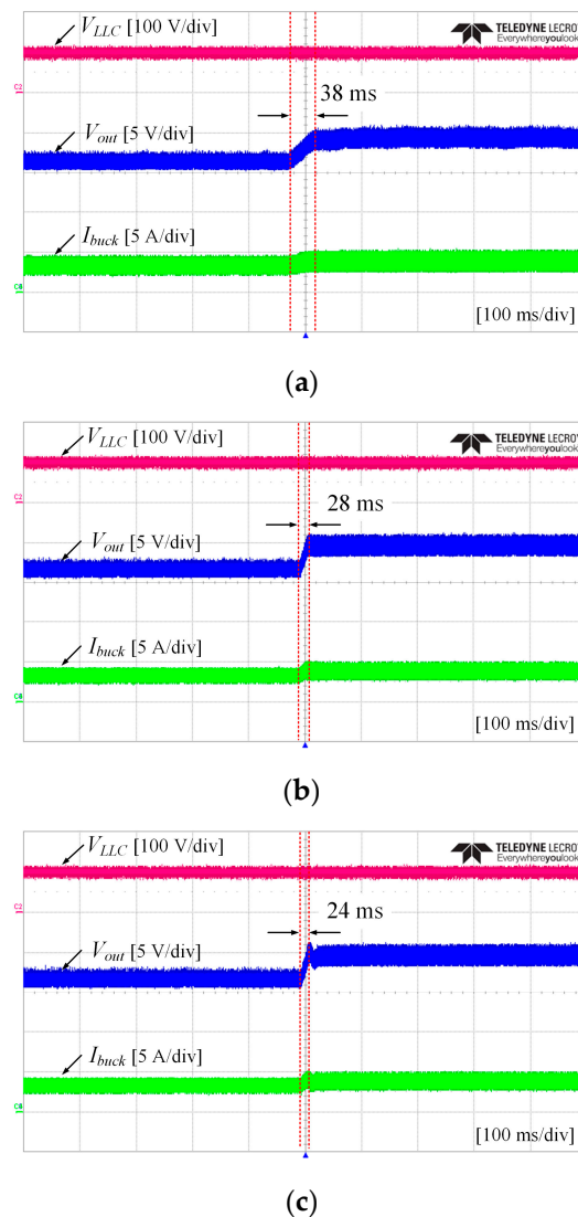
Figure 18. Experiment results of the proposed RBFLC method for different values of \eta : (a) \eta is 0.01; (b) \eta is 0.05; (c) \eta is 0.1.
