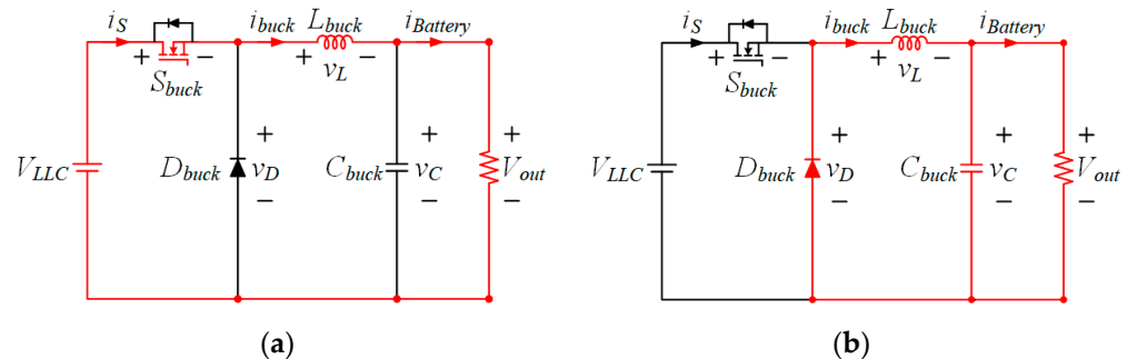
Figure 2. Operating principle of the buck converter: (a) Mode 1; (b) Mode 2.
