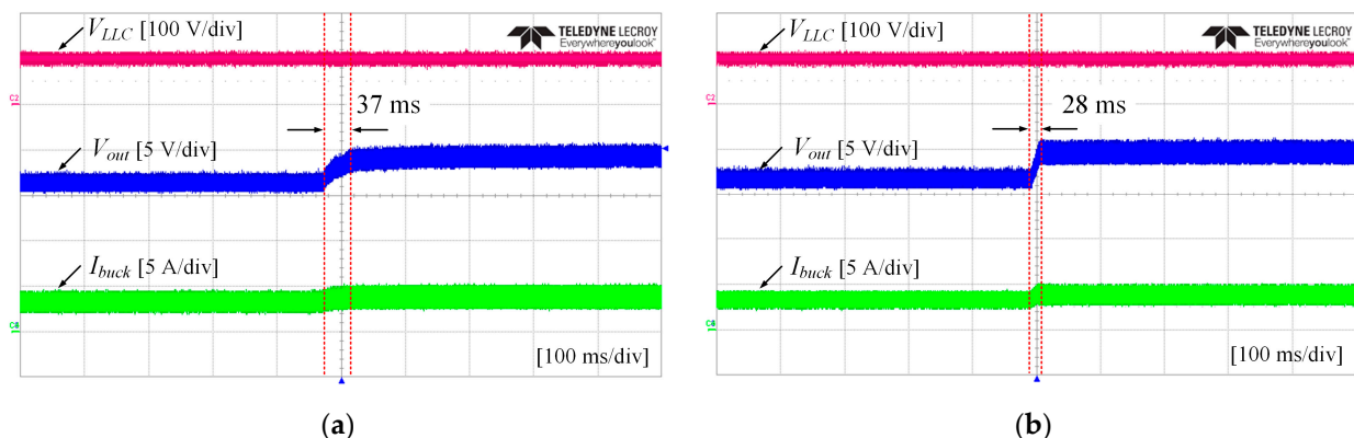
Figure 17. Experimental results of transient state responses: (a) PI controller; (b) proposed RBFLC.
