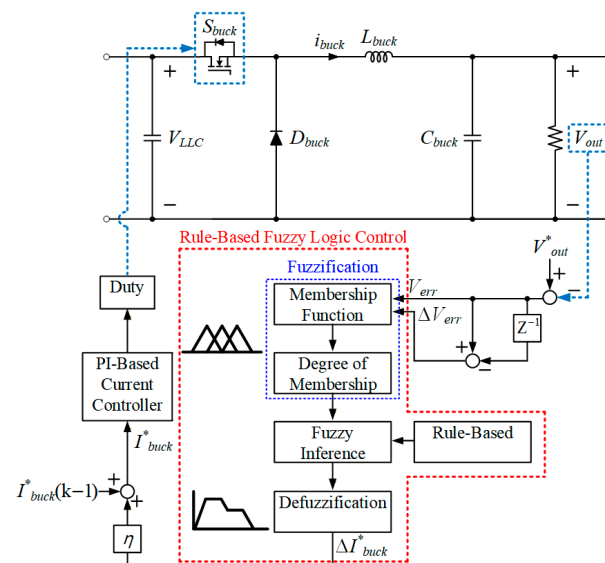
Figure 3. Control block diagram of the RBFLC method.
