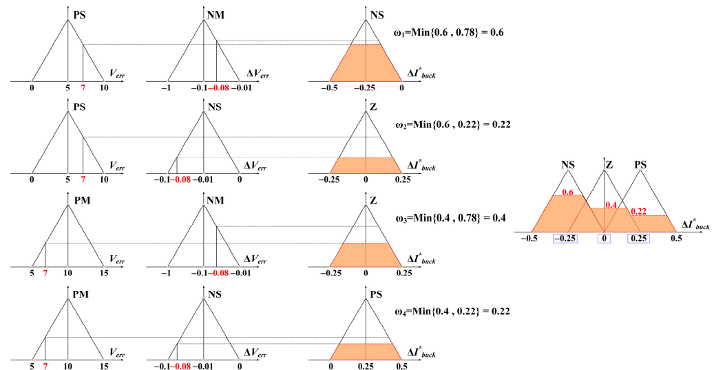
Figure 8. Fuzzy inference process.
