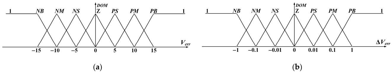
Figure 5. Membership function of (a) V_{err} ; (b) \Delta V_{err} .
