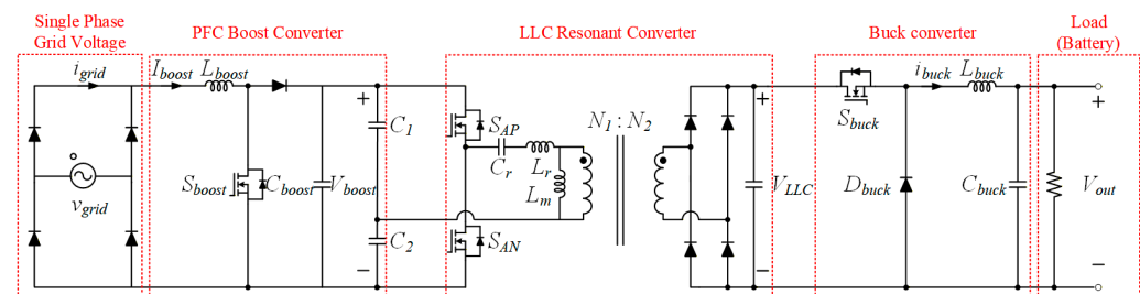
Figure 1. Topology of the power conversion stages of the PMD battery charger.
