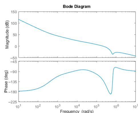
Figure 9. Bode diagram of the transfer function G(s) .
