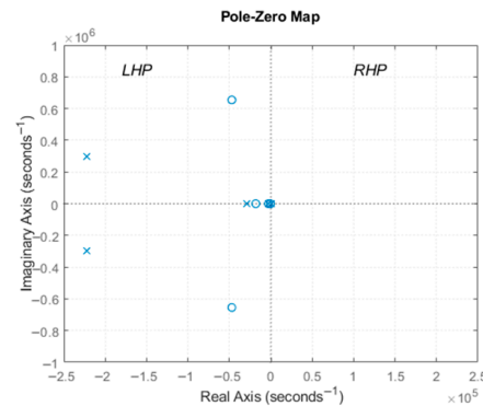
Figure 10. Pole-zero map of the transfer function G(s) on complex plane.
