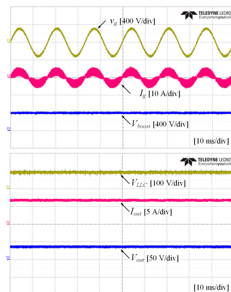
Figure 15. Various experimental results of the PMD battery charger.
