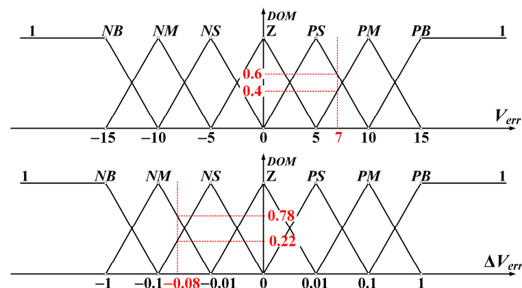
Figure 6. Calculation process of DOM using the membership function when V_{err} is 7 and \Delta V_{err} is -0.08 .
