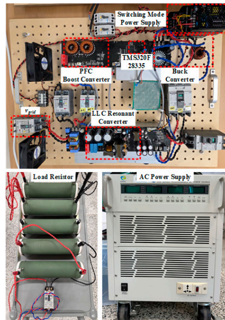
Figure 14. Experimental setup.
