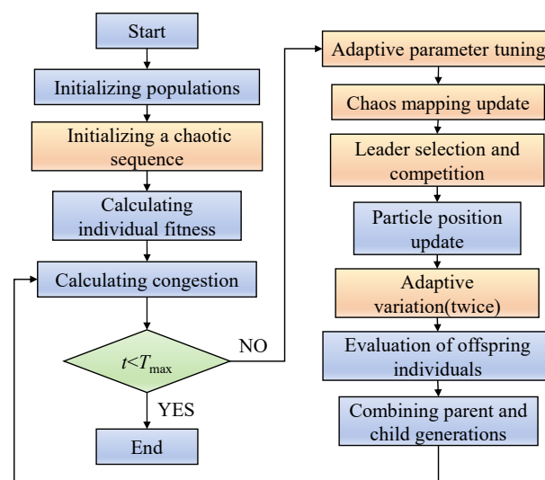
Figure 7. Improved multi-objective particle swarm algorithm flow.
