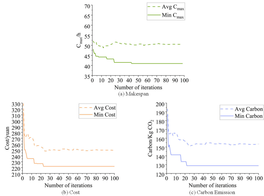
Figure 9. Iterative convergence curves for different objectives.
