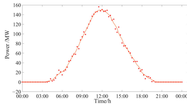
Figure 1. Photovoltaic power output curve.
