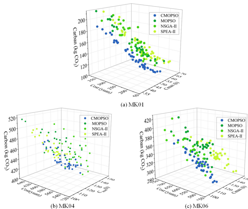
Figure 14. Comparison of different algorithmic Pareto fronts.
