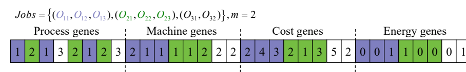
Figure 5. Four-layer coding scheme.
