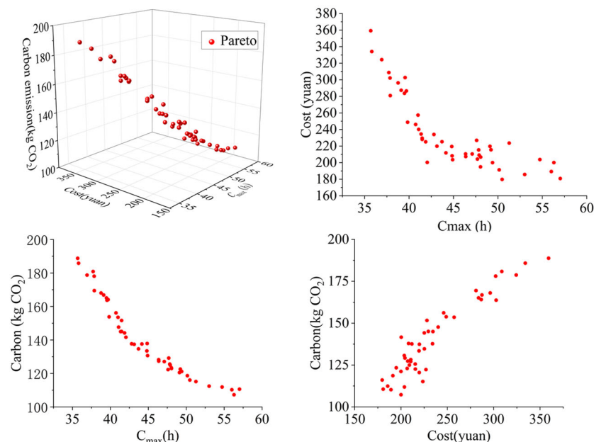
Figure 8. Pareto frontier based on the triple objective.
