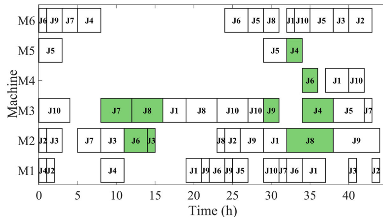
Figure 10. Scheduling results of the balanced program.
