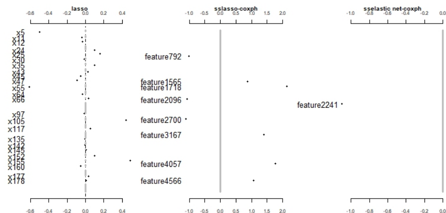
Figure 4. Cox coefficient estimates plot for the genes selected in DBCD Data.
