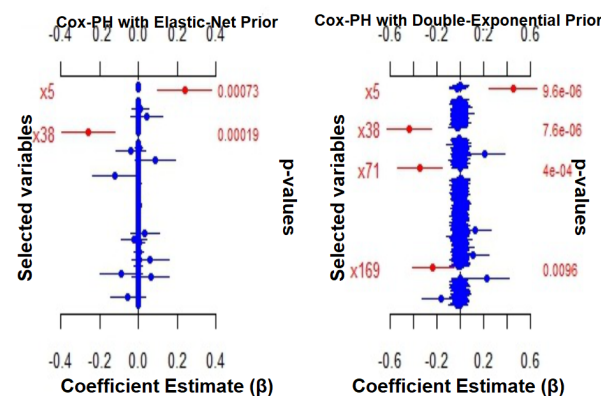
Figure 1. Estimated regression coefficients from the Bayesian Cox proportional hazards model under hierarchical elastic net and double-exponential (Laplace) priors for Scenario 1. Red points indicate posterior mean estimates, while blue lines represent 95% credible intervals.
