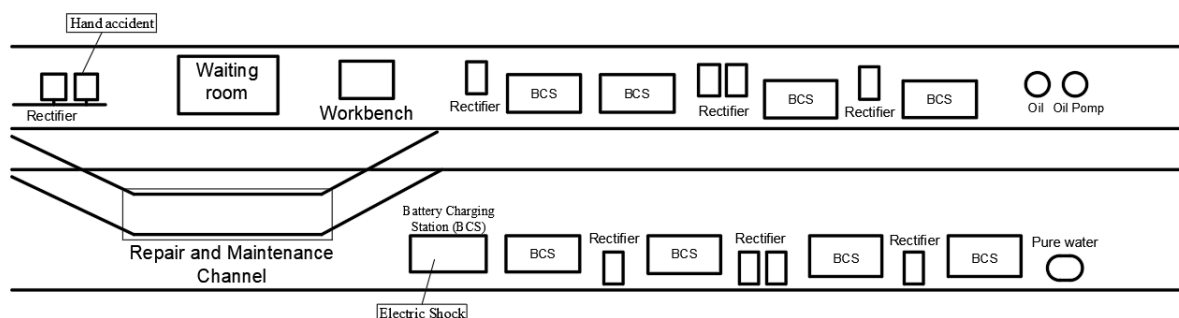
Figure 2. Battery charging station layout plan.
