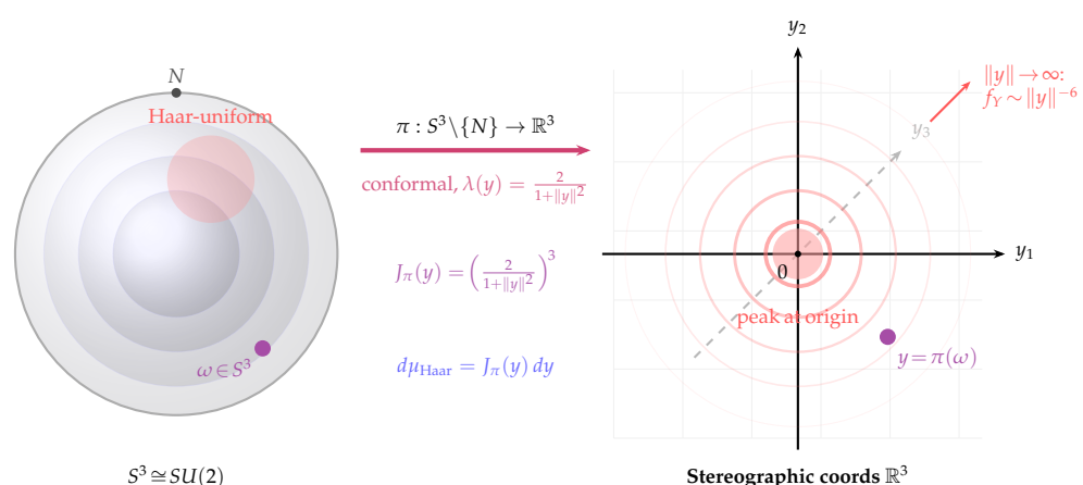
Figure A1. Stereographic projection \pi : S^3 \setminus \{N\} \rightarrow \mathbb{R}^3 and the induced reference-measure distortion. A Haar-uniform intrinsic distribution becomes nonuniform in coordinates solely through the chart-volume factor J_\pi(y) = \left(\frac{2}{1+|y|^2}\right)^3 . The heavy tail f_Y \sim \|y\|^{-6} is a coordinate artifact; the intrinsic distribution on S^3 remains uniform.
