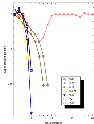
Figure 4. Computational outcomes for the MSR obtained in Experiment 1 with n = 250 .
