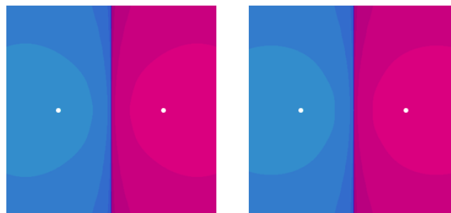
Figure 2. Attraction basins for (25) in left and (27) in right.
