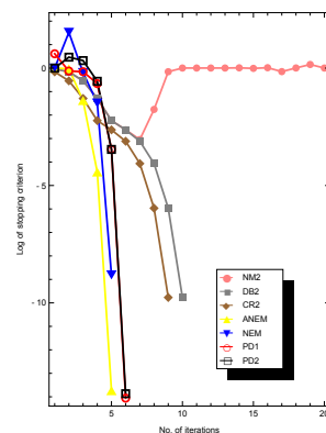
Figure 5. Numerical outcomes for the MSR obtained in Experiment 1 with n = 550 .
