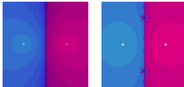
Figure 1. Attraction basins for (9) in left and Padé 1–4 in right.
