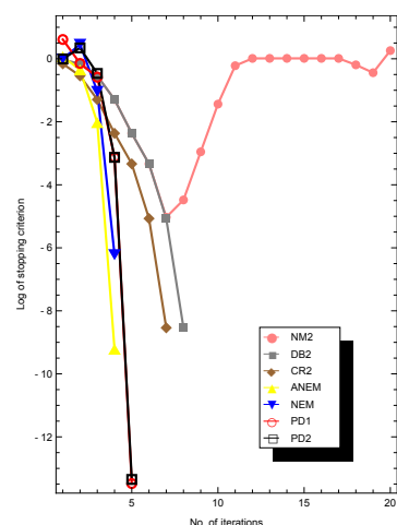
Figure 3. Numerical outcomes for the MSR obtained in Experiment 1 with n = 150 .
