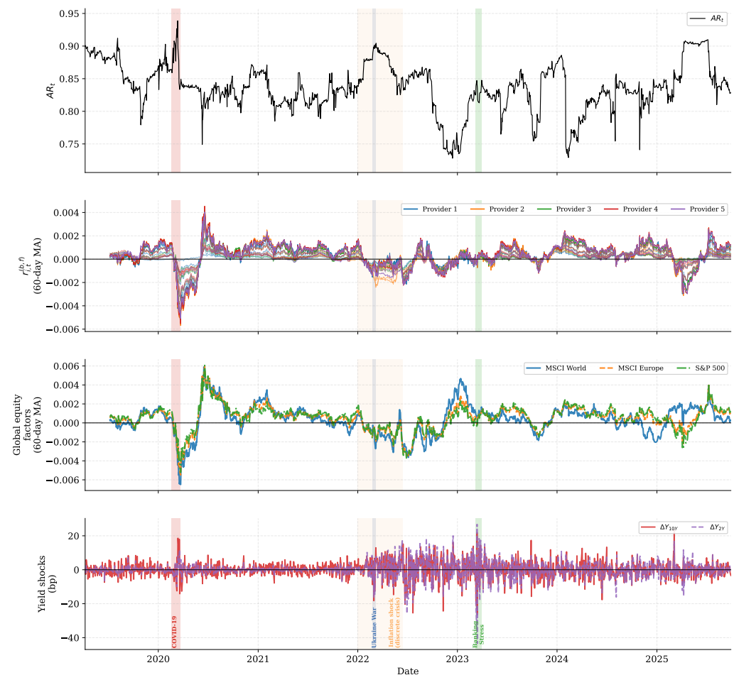
Figure 3. Panel 1: Baseline absorption ratio \{AR_t\} computed from R^{(f)} using a 60-day rolling covariance matrix. Panel 2: Sixty-day moving averages of all fund-specific benchmark returns R^{(b,f)} . Panel 3: Global equity factors (MSCI World, MSCI Europe, and S&P 500). Panel 4: Euro-area yield shocks based on daily changes in 10-year and 2-year AAA sovereign yields. Shaded regions denote major market stress episodes. The absorption ratio is constructed exclusively from pension-fund returns; benchmark and macro-financial series are included for interpretation only.
