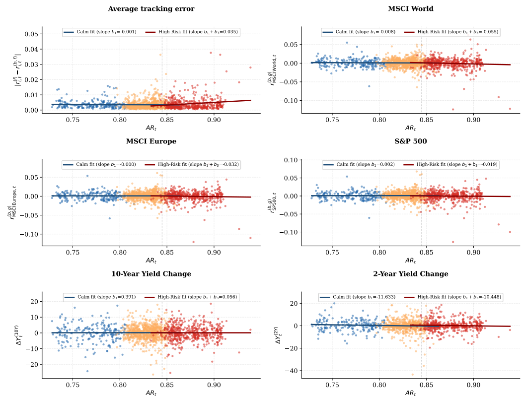
Figure 11. Regime-conditional scatter of AR_t against each interpretive series. The blue line is fitted only to non-high observations (slope b_1 ); the dark red line only to High-Concentration observations (slope b_1 + b_3 ), each over the AR_t range observed within its regime. The vertical dotted line marks the crisis threshold \tau = 0.845 . Coefficients and HAC p -values are in Table 19.
