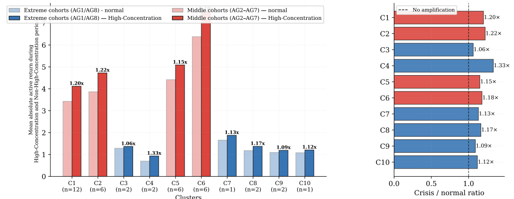
Figure 12. Mean absolute active return by cluster under Non-High and High-Concentration regimes (left panel) and the crisis amplification ratio (right panel), defined as the mean absolute active return on High-Concentration days divided by that on non-high days. Red bars denote middle-cohort (growth) clusters AG2–AG7; blue bars denote extreme-cohort (conservative) clusters AG1 and AG8/TIPF. Light shading = non-high regime; dark shading = High-Concentration regime.
