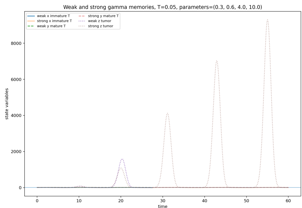
Figure 3. Case A at T = 0.05 : increasing the mean memory produces larger excursions. The plot is retained as a transient simulation; it does not assert convergence to a bounded attractor.
