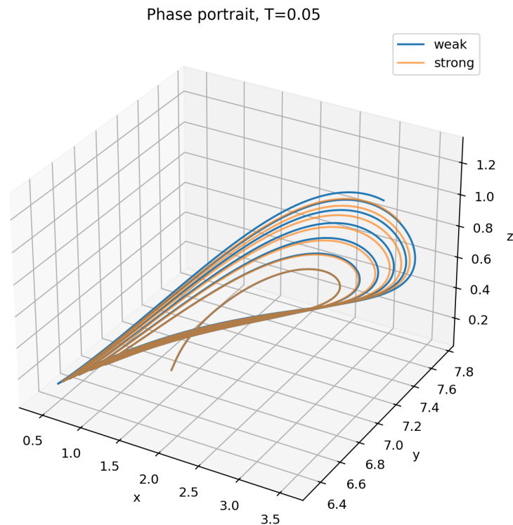
Figure 6. Case B at T = 0.05 : post-threshold phase portrait. The trajectory no longer contracts to E_2 , providing a geometric counterpart to the positive spectral abscissa.
