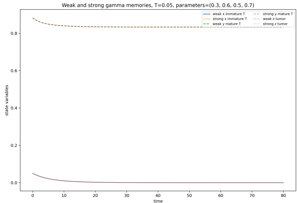
Figure 7. Case D at T = 0.05 : tumor-free stabilization. The tumor component decreases toward zero while the mature immune component approaches the tumor-free level.
