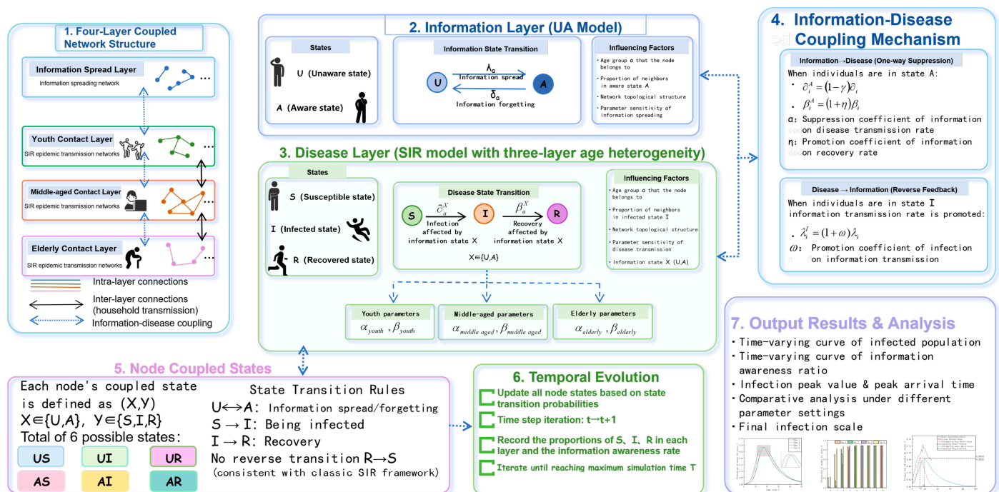
Figure 3. UA-SIR Information-Disease Coupled Propagation Model Flowchart.
