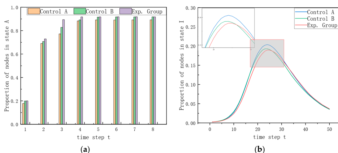
Figure 5. Comparison between the experimental group and the control groups. (a) Partial view of the information awareness rate ( A(t) ) over time (day). Only the early and middle stages are shown because the awareness rate changes only slightly after reaching a relatively stable level in the later stage. (b) Evolution curves of the infection proportion ( I(t) ) in the disease transmission process. Control A adopts unified information diffusion parameters, Control B introduces age-specific information diffusion parameters, and the experimental group further incorporates the infection-induced feedback mechanism.
