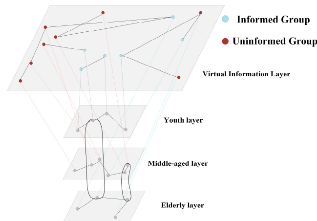
Figure 2. The four-layer information–disease-coupled heterogeneous mixed network proposed in this work, containing one virtual information layer and three age-based disease transmission layers (youth, middle-aged, elderly layers, with gray nodes representing individuals belonging to different age groups). Light blue nodes stand for informed individuals and dark red nodes stand for uninformed individuals in the information layer; straight lines between layers represent the coupling connections of information and disease spread. Each physical individual node in the three age layers has a one-to-one corresponding node in the virtual information layer, and the vertical connecting lines indicate the mapping relationship between physical nodes and information nodes.
