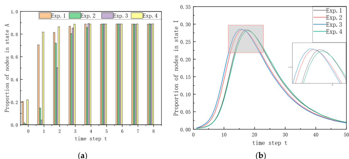
Figure 8. Sensitivity analysis of initial information seed locations. (a) Partial view of the information awareness rate ( A(t) ) under different initial information seed locations. Only the early and middle stages are shown because the curves change only slightly after reaching a relatively stable level in the later stage. (b) Evolution curves of the infection proportion ( I(t) ) in the disease transmission process under different seed-location strategies. Experiments 1–4 correspond to information seeds initially placed in the middle-aged layer, youth layer, older-adult layer, and mixed-age layers, respectively.
