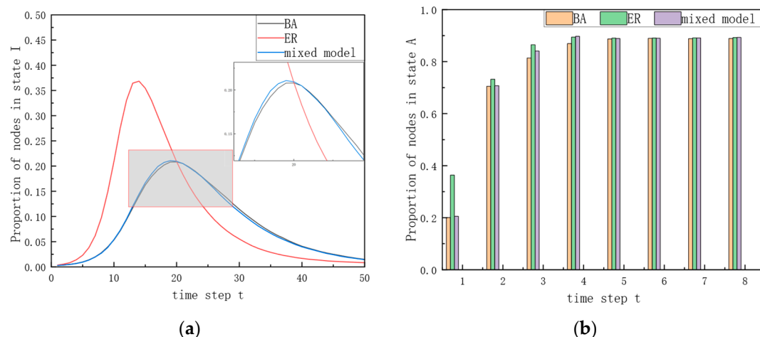
Figure 9. Sensitivity analysis of network topology. (a) Evolution curves of the infection proportion ( I(t) ) in the disease transmission process under different network topologies. (b) Partial view of the information awareness rate ( A(t) ) under different network topologies. Only the early and middle stages are shown because the curves change only slightly after reaching a relatively stable level in the later stage. BA denotes the case in which all three age layers adopt BA scale-free networks, ER denotes the case in which all three age layers adopt ER random networks, and the mixed model denotes the case in which the youth and middle-aged layers adopt BA networks while the older-adult layer adopts an ER network.
