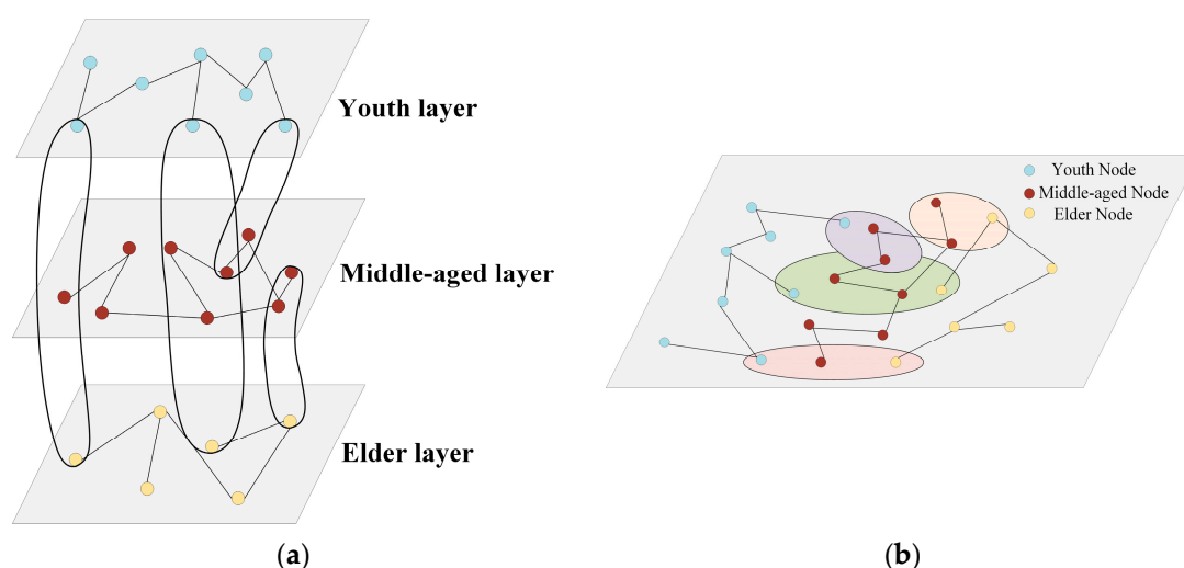
Figure 1. Age-family hyperedge multilayer heterogeneous network structure. (a) 3D schematic of the three-layer network with youth, middle-aged, and elderly age groups connected via household hyperedges; (b) Top view of the age-stratified multilayer network with household hypergroup clusters.
