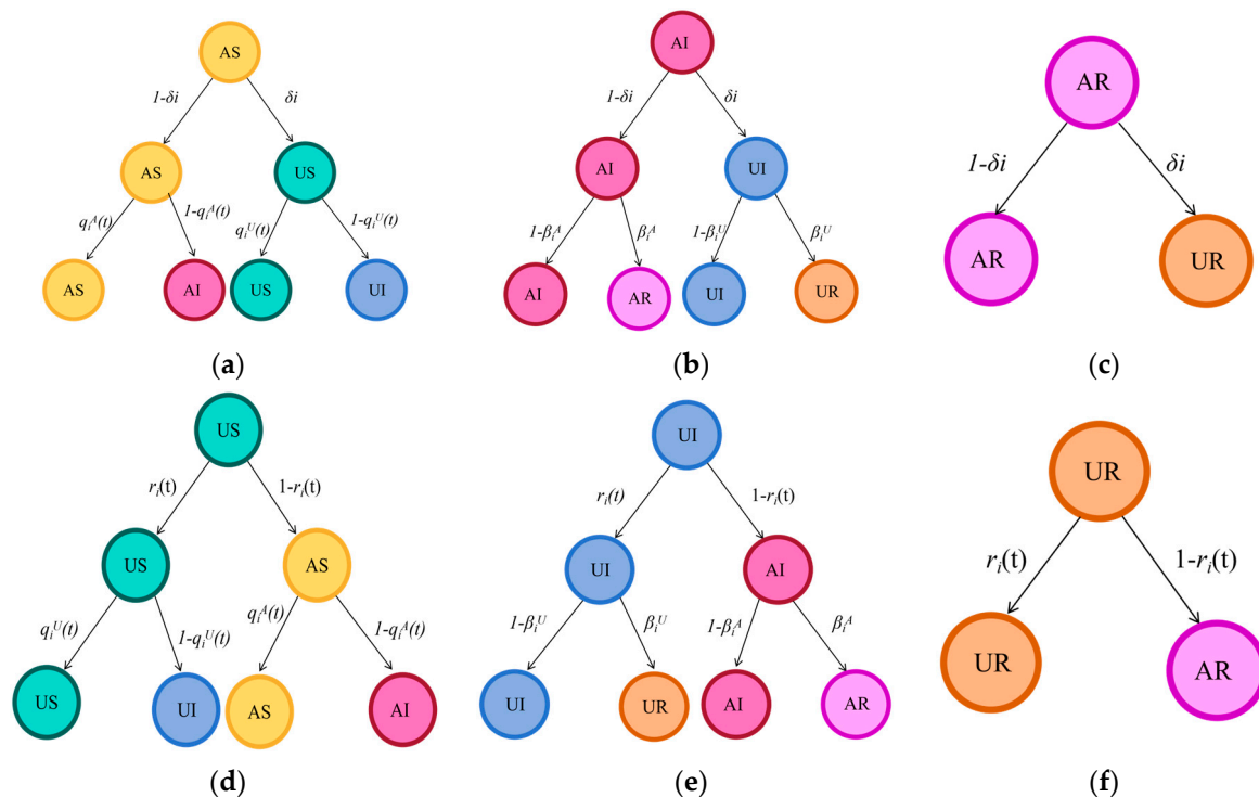
Figure 4. State transition probability tree. Panels (a–f) show the transition paths starting from the six coupled states (AS), (AI), (AR), (US), (UI), and (UR), respectively. The transition probabilities include information acquisition 1 - r_i(t) , information forgetting \delta i , disease infection 1 - q_i^A(t) or 1 - q_i^U(t) , and recovery \beta_i^U or \beta_i^A , depending on the information and disease states of the node.
