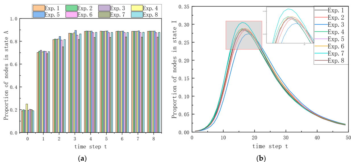
Figure 7. Sensitivity analysis of the information-spreading rate \lambda and forgetting rate \delta . (a) Partial view of the information awareness rate ( A(t) ) under different parameter settings. Only the early and middle stages are shown because the curves change only slightly after reaching a relatively stable level in the later stage. (b) Evolution curves of the infection proportion ( I(t) ) in the disease transmission process under different parameter settings. Experiments 1–8 correspond to different adjustments of the information-spreading rate and forgetting rate in the youth, middle-aged, and older-adult layers.
