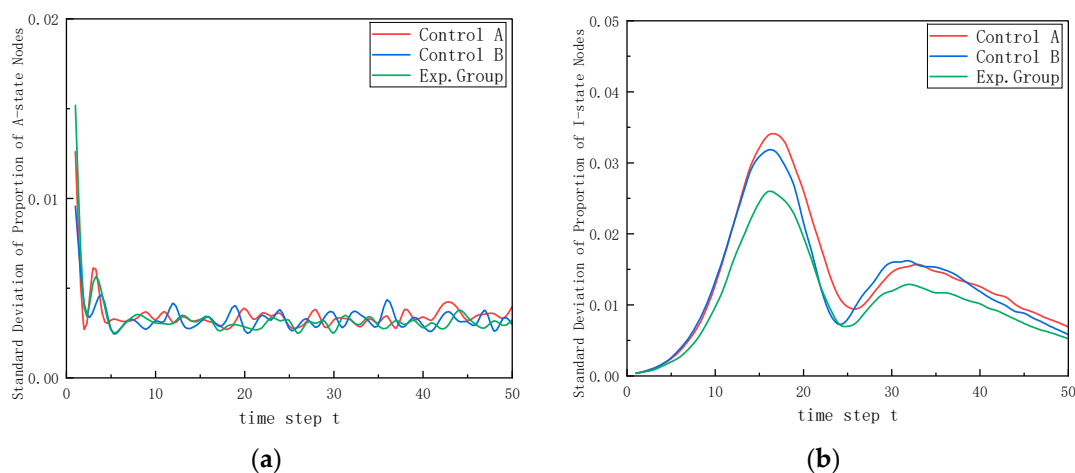
Figure 6. Stochastic variability of the coupled spreading dynamics. (a) Standard deviation of the aware proportion; (b) Standard deviation of the infected proportion. The standard deviations were calculated from 50 independent Monte Carlo realizations.
