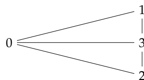
Figure 1. Graph of G(A) .
