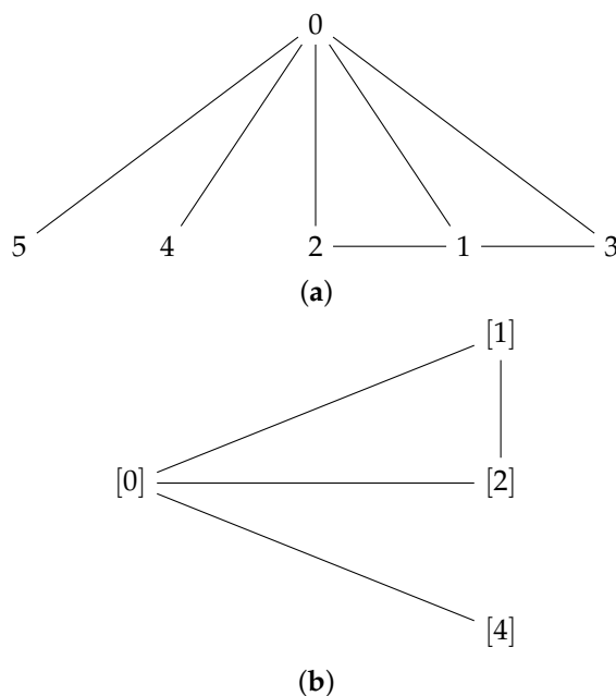
Figure 2. (a) Graph of G(A) ; (b) graph of G_E(A) .
