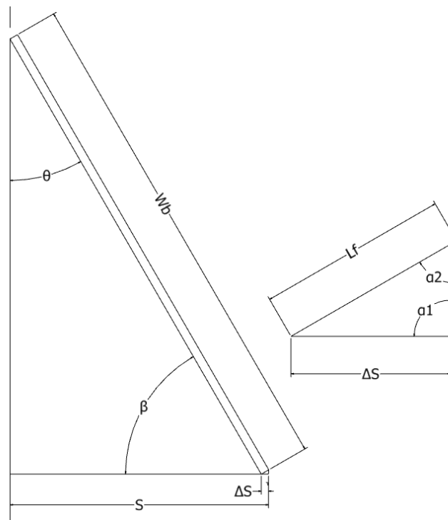
Figure 4. Heat exchanger width formulation.
