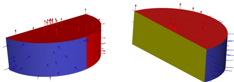
Figure 7. Boundary conditions.
