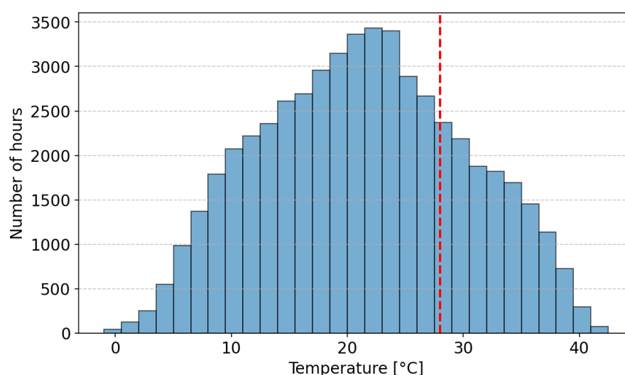
Figure 3. Hourly ambient temperature distribution for Upington (2017–2022).
