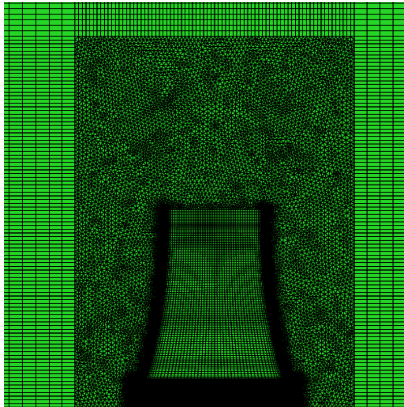
Figure 10. Surrounding mesh.
