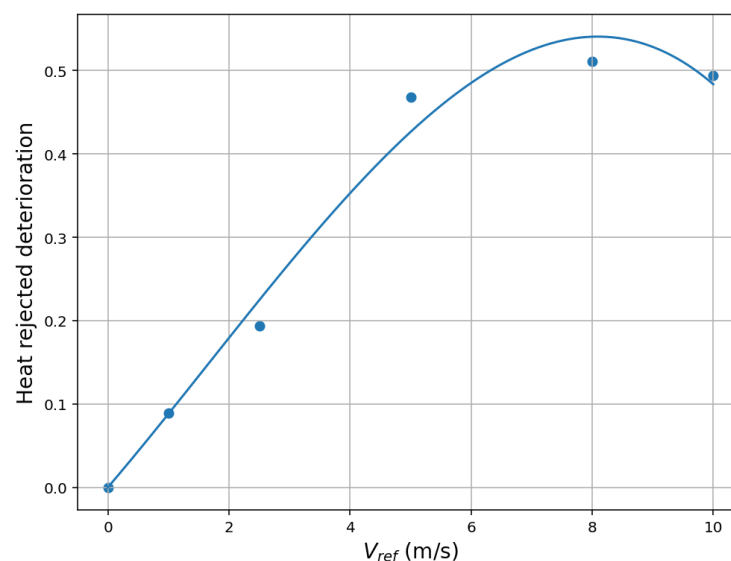
Figure 11. Effect of wind on heat rejection rate.
