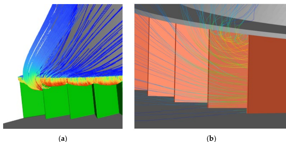
Figure 14. Recirculation phenomenon: (a) current work; (b) Strydom et al. [16].
