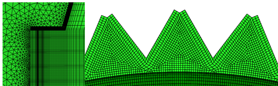
Figure 9. Heat exchanger mesh.
