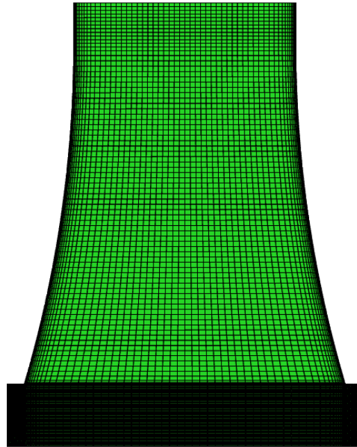
Figure 8. Tower mesh.
