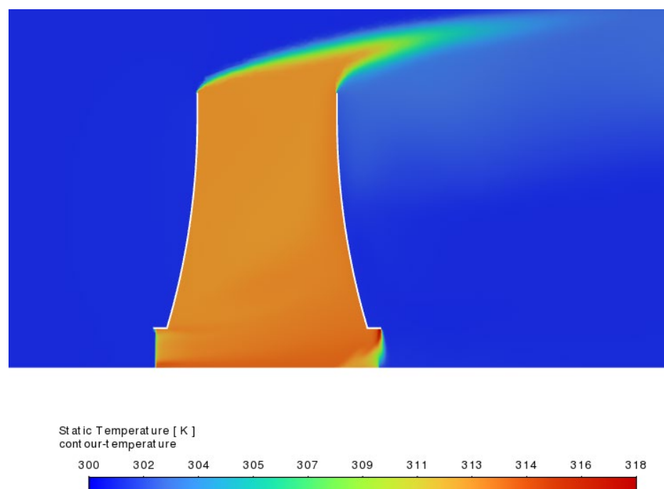
Figure 17. Side profile static temperature contour plot of NDACC under 10 m/s crosswind.
