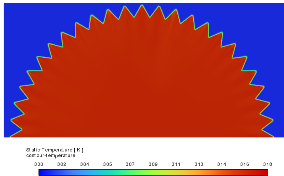
Figure 18. Cross-section static temperature contour plot of NDACC under no-wind conditions.
