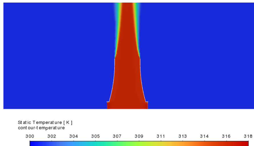
Figure 16. Side profile static temperature contour plot of NDACC under no-wind conditions.
