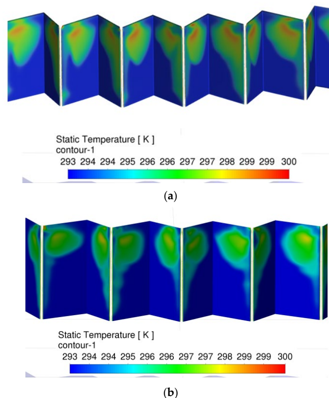
Figure 15. Localized heat exchanger hot spots phenomenon: (a) current work; (b) Strydom et al. [16].
