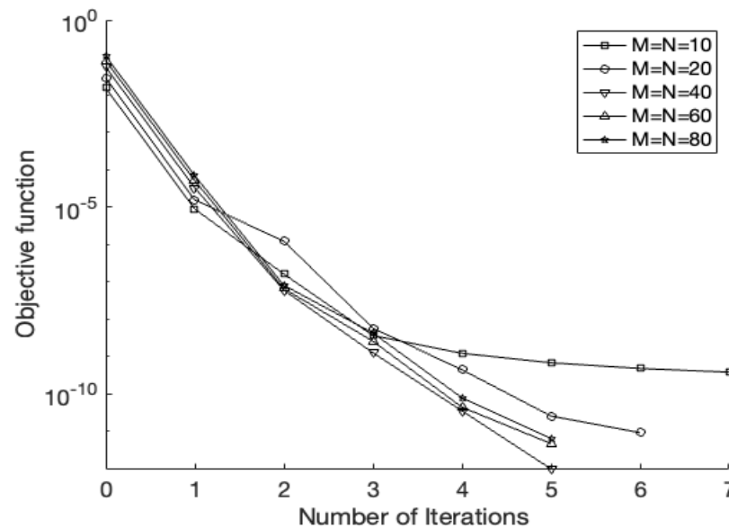
Figure 15. The objective function (40), without regularized \vartheta = 0 , and p = 0 noise for Example 2 at various mesh sizes M = N = \{10, 20, 40, 60, 80\} .
