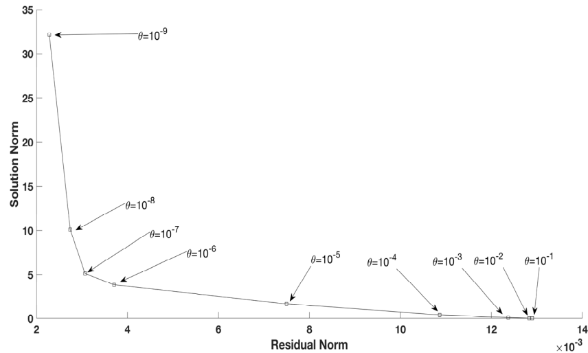
Figure 11. The L-curve plot with various regularization when p = 0.1\% noise for Example 1.
