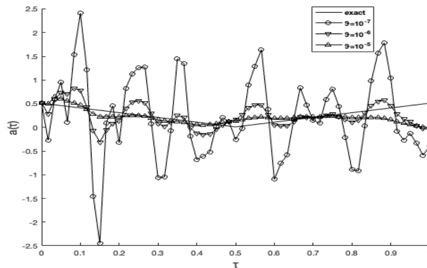
Figure 18. Accurate and approximate solution for the non-smooth potential term a(\tau) with \vartheta \in \{10^{-7}, 10^{-6}, 10^{-5}\} and p = 0.1\% noise for Example 2.
