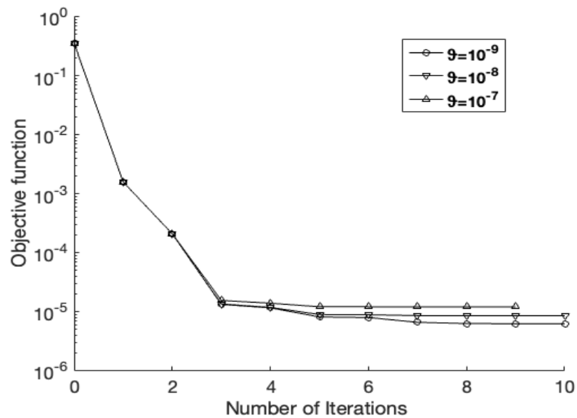
Figure 12. The minimized objective functional (40), with \theta \in \{10^{-9}, 10^{-8}, 10^{-7}\} and p = 0.1\% noise amount percentage for Example 1.
