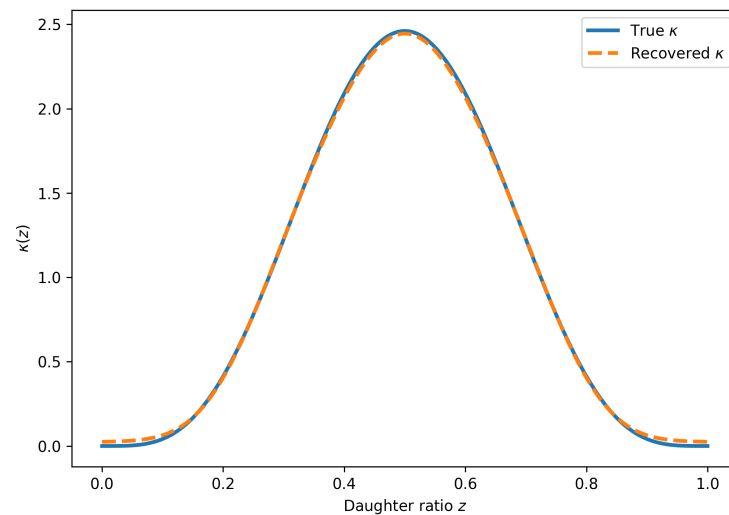
Figure 3. Synthetic inverse test with known B : recovery of the daughter distribution \kappa(z) .
