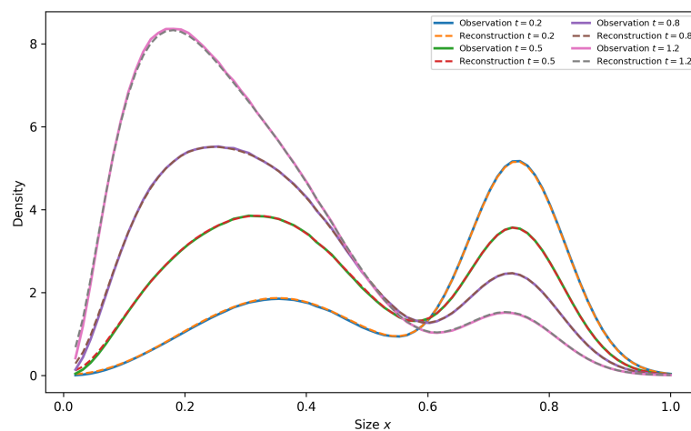
Figure 4. Synthetic inverse test with known B : comparison between true and reconstructed particle-size distributions.
