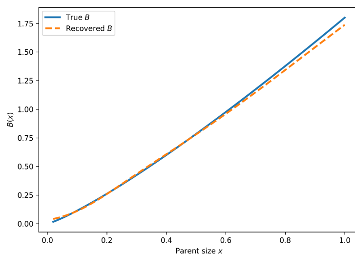
Figure 7. Joint synthetic inverse test: recovery of the breakup rate B(s) .
