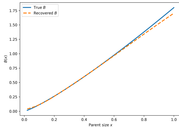
Figure 5. Synthetic inverse test with known \kappa : recovery of the breakup rate B(s) .
