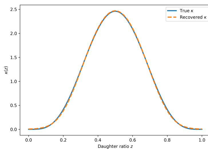
Figure 8. Joint synthetic inverse test: recovery of the daughter distribution \kappa(z) .
