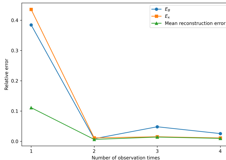
Figure 14. Effect of the number and temporal placement of the observed particle-size distributions on the joint recovery of B and \kappa in the unimodal benchmark. The cases use one observation at t = 0.8 , two observations at t = 0.5, 1.2 , three observations at t = 0.2, 0.8, 1.2 , and four observations at t = 0.2, 0.5, 0.8, 1.2 . The figure reports the relative errors E_B and E_\kappa , together with the mean reconstruction error; all remaining numerical settings and the ground-truth fragmentation law are kept unchanged.
