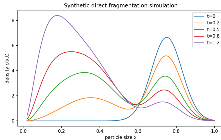
Figure 1. Synthetic direct fragmentation simulation. The initial distribution is concentrated near large sizes, and the evolution shows the progressive production of smaller fragments.
