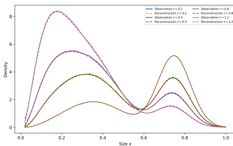
Figure 9. Joint synthetic inverse test: comparison between true and reconstructed particle-size distributions.
