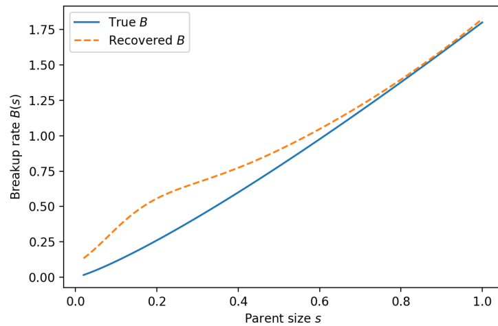
Figure 10. Bimodal synthetic test: recovery of the breakup rate B(s) .
