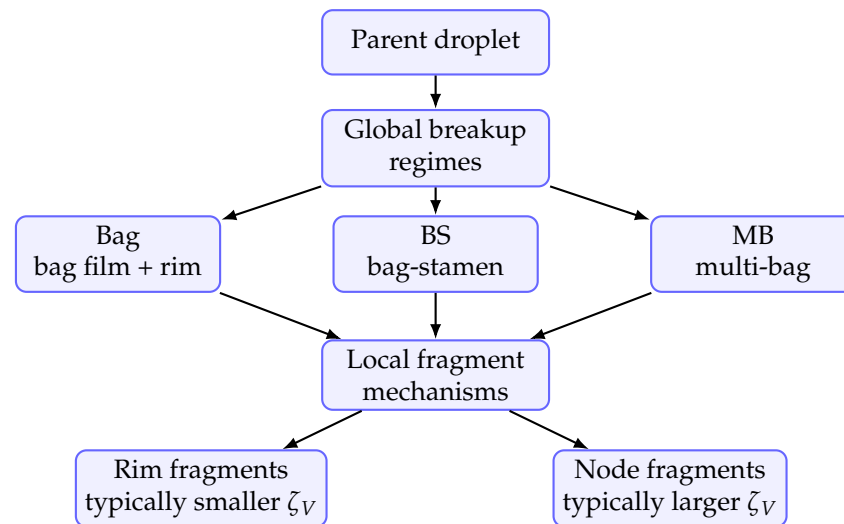
Figure 15. Conceptual schematic of the breakup-regime and fragment-mechanism labels used in the experimental analysis.
