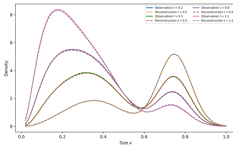
Figure 6. Synthetic inverse test with known \kappa : comparison between true and reconstructed particle-size distributions.
