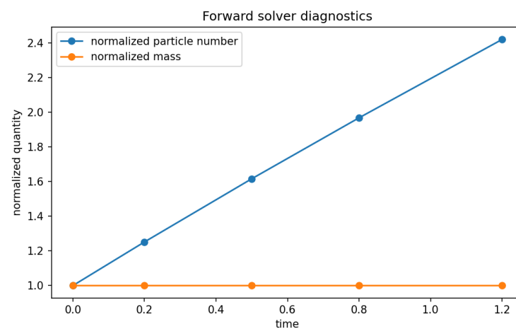
Figure 2. Forward solver diagnostics. The total particle number increases, while the total mass remains conserved.
