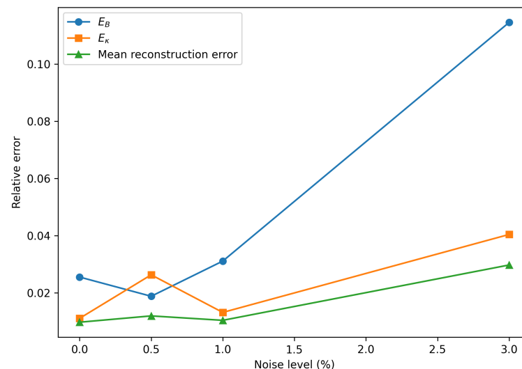
Figure 13. Robustness of the joint neural inverse recovery of B and \kappa in the unimodal benchmark for relative noise levels 0%, 0.5%, 1%, and 3%. Independent Gaussian perturbations are scaled by the maximum value of the distribution at each observation time, as defined in (44), and negative perturbed values are projected to zero. The figure reports the relative errors E_B and E_\kappa , together with the mean reconstruction error; all remaining numerical settings are unchanged from the noise-free joint-recovery experiment.
