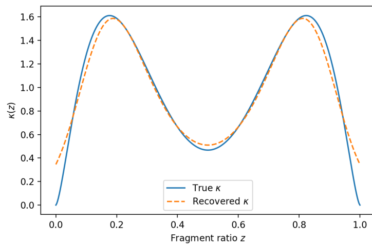
Figure 11. Bimodal synthetic test: recovery of the bimodal daughter distribution \kappa(z) .
