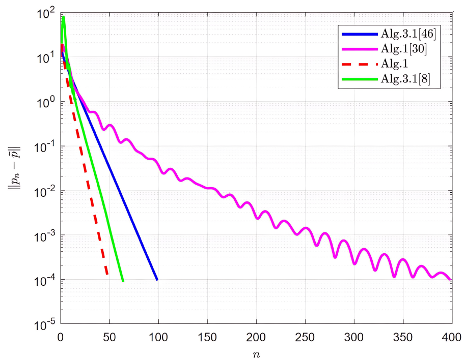
Figure 2. Number of iterations ( n ) for Example 1 ( m = 400, \varepsilon = 10^{-4} ).
