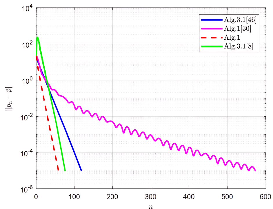
Figure 3. Number of iterations ( n ) for Example 1 ( m = 500, \varepsilon = 10^{-5} ).
