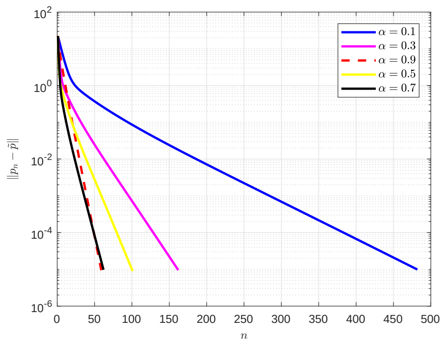
Figure 1. The sensitivity analysis of \alpha for Algorithm 1 and number of iterations ( n ) for Example 1.
