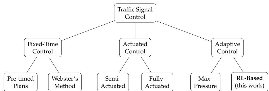
Figure 2. Classification of traffic signal control methods. RL-based control belongs to the adaptive category, as it continuously adjusts signal phases in response to observed traffic conditions.
