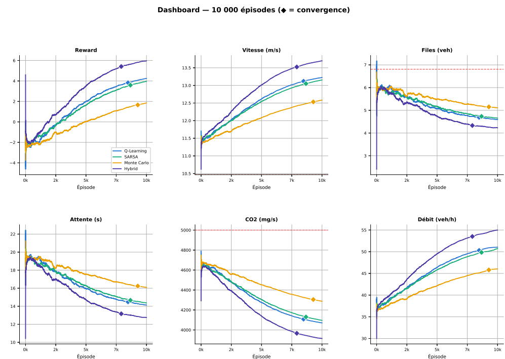
Figure 11. Performance dashboard: reward, speed, queue length, waiting time, CO 2 emissions, and throughput for all four algorithms. The marker ♦ indicates the convergence episode t^* .
