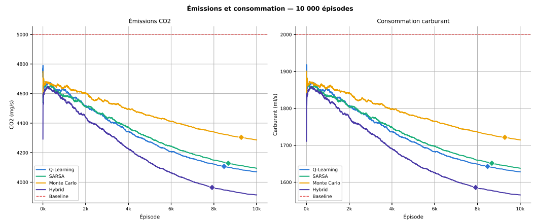
Figure 9. Evolution of CO 2 emissions (left) and fuel consumption (right). Red dashed lines indicate baseline values (5000 mg/s and 2000 mL/s).
