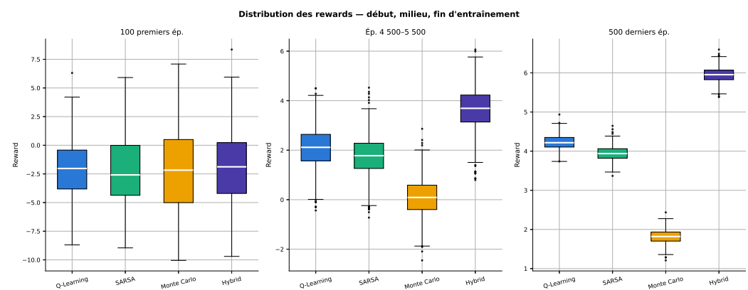
Figure 10. Box plots of reward distributions: early (episodes 1–100), mid (episodes 4500–5500), and late (episodes 9500–10,000).
