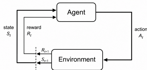
Figure 1. The agent–environment interaction in RL applied to traffic signal control.
