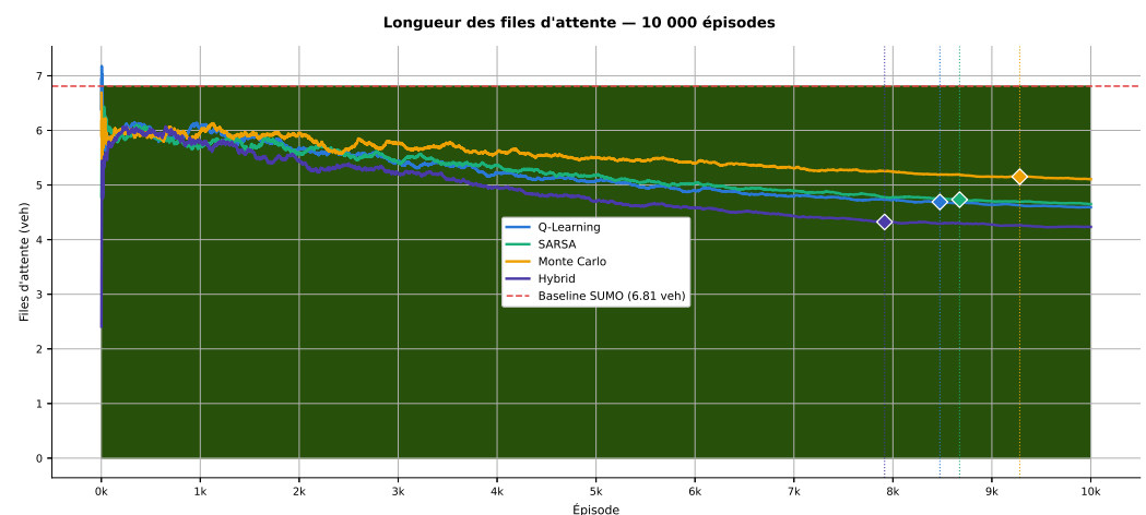
Figure 8. Evolution of mean queue length. The red dashed line indicates the SUMO baseline (6.81 veh).
