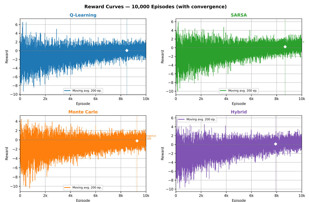
Figure 4. Learning curves (200-episode moving average) for the four algorithms over 10,000 training episodes. The marker \blacklozenge denotes the convergence episode t^* .
