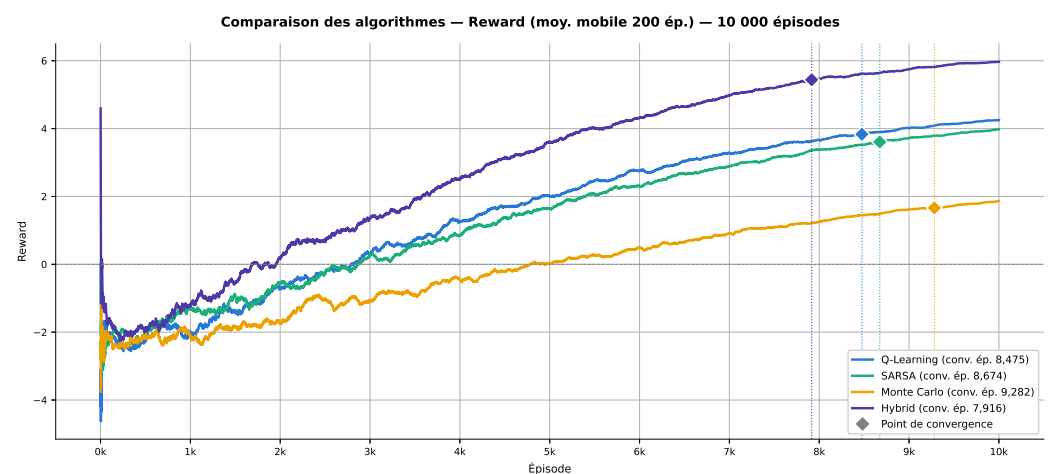
Figure 5. Comparison of the smoothed reward curves for all four algorithms over 10,000 episodes.
