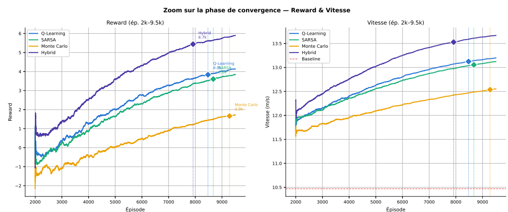
Figure 6. Zoomed view of the convergence phase (episodes 2000–9500): reward ( left ) and mean vehicle speed ( right ). Vertical dashed lines indicate t^* for each algorithm.
