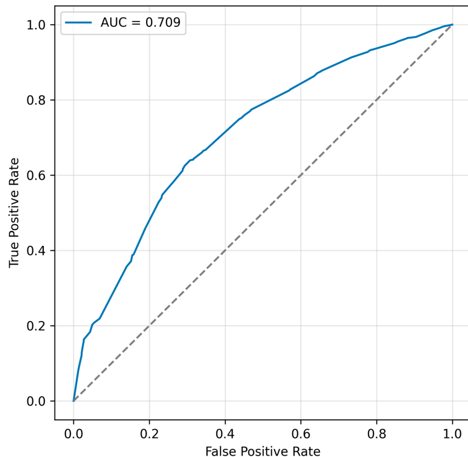
Figure 3. ROC curve of multivariable logistic regression model's CPR outcomes.
