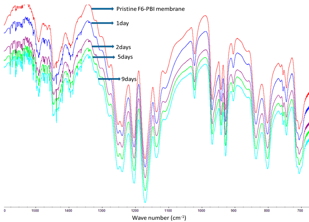
Figure S2. FT-IR spectrum of F6-PBI membrane as a function of sulfuric acid doping time (30% sulfuric acid at room temperature).
