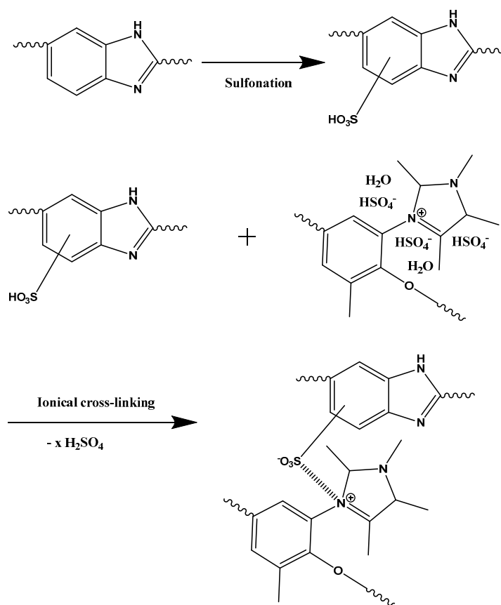
Figure S1. Possible loss of \text{H}_2\text{SO}_4 during the sulfonation of PBI based blend membranes.
