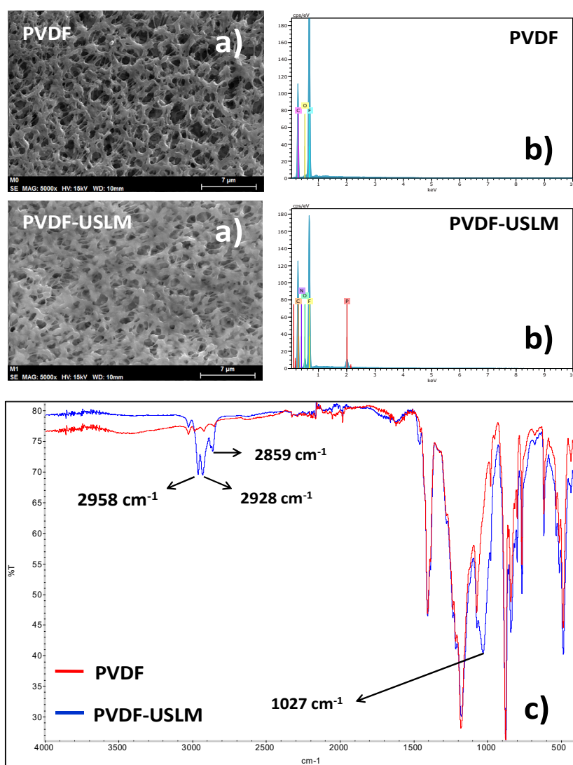
Figure 3. Membrane characterization of PVDF and PVDF-USLM by (a) SEM; (b) EDX; (c) FTIR.
